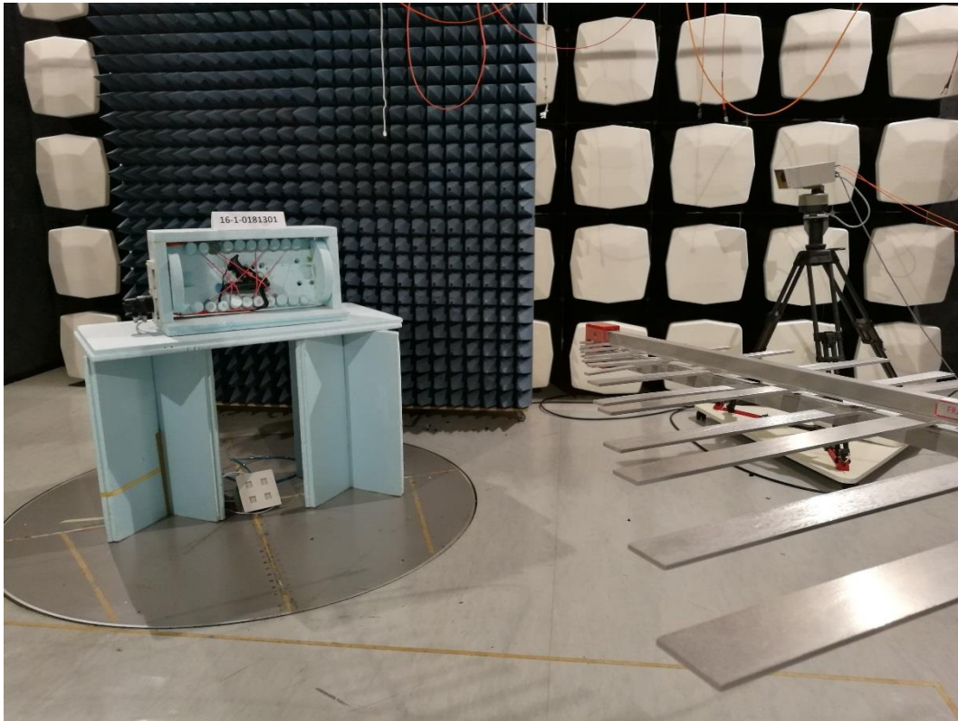
Photograph 14: Set Up 1-Overall View-30 MHz-1 GHz - EUT Laying 90° - Front Side
