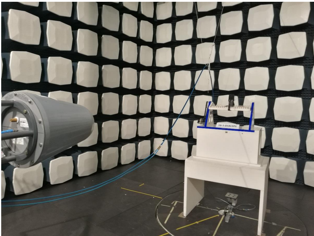
Photograph 19: Set Up 1-Overall View - above 1 GHz - EUT Standing 0° - Front Side
