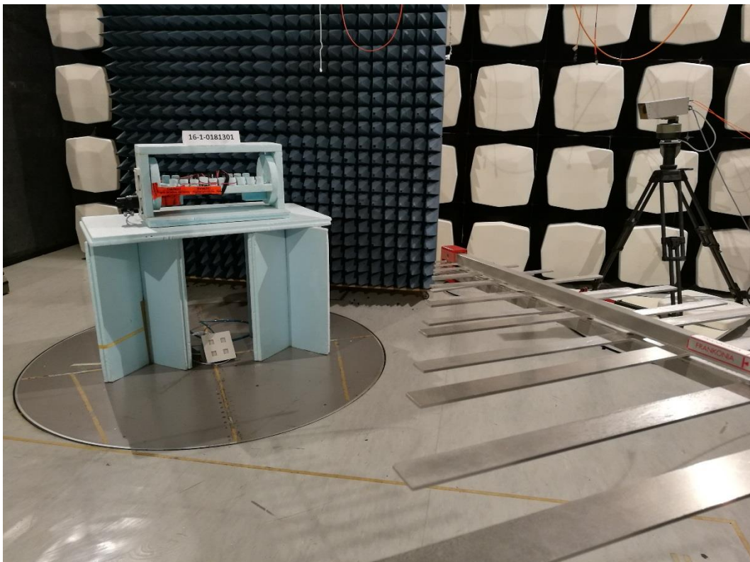
Photograph 15: Set Up 1-Overall View - 30 MHz-1 GHz - EUT Laying 0° - Front Side
