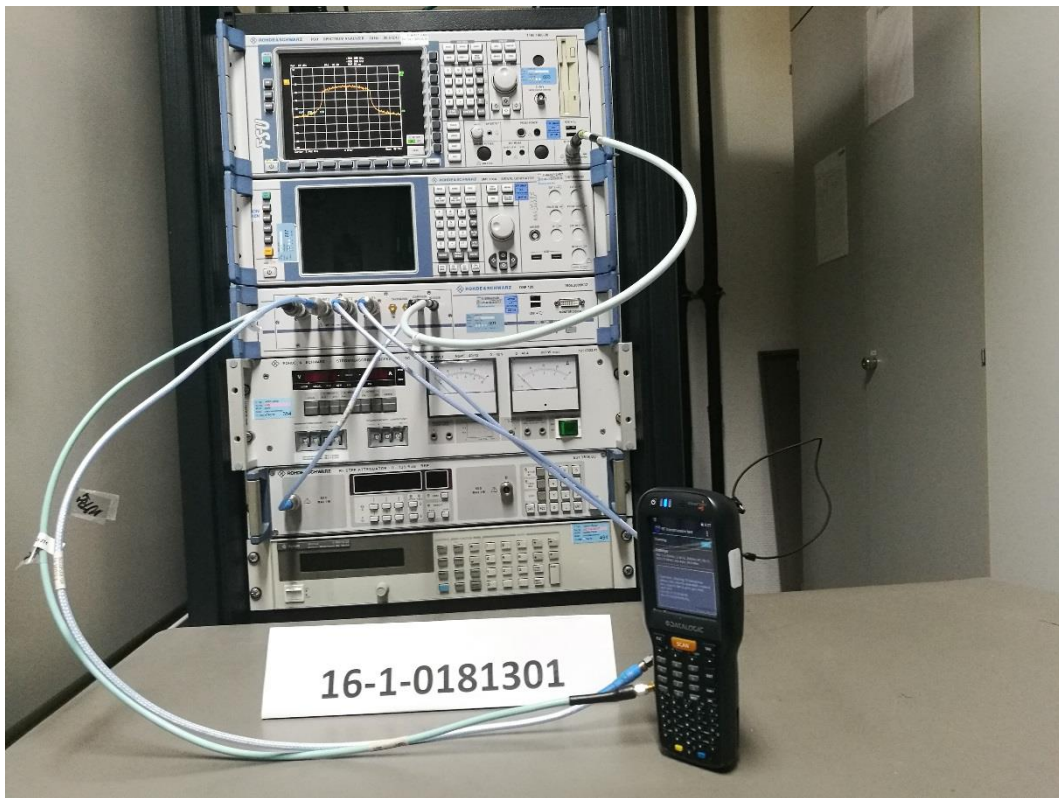
Photograph 3: Set Up 2-Overall View- ANT1 + ANT2 used [WLAN n Mode-MIMO]
