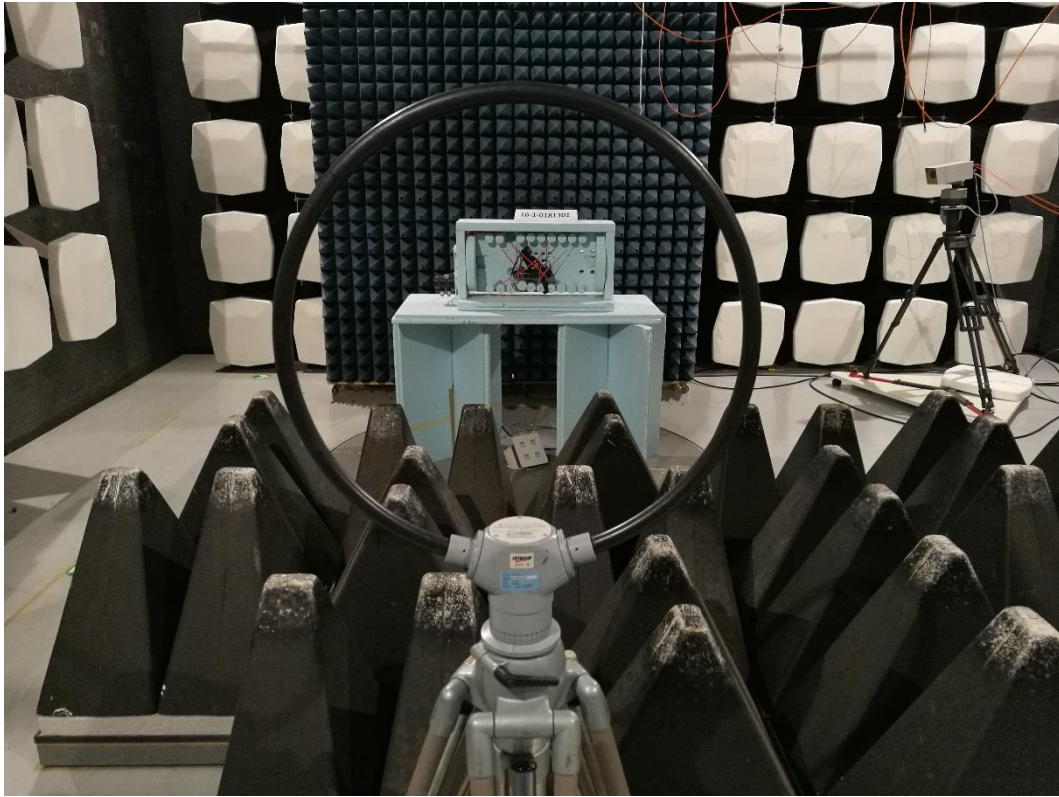
Photograph 10: Set Up 1-Overall View- 9 kHz-30 MHz- EUT Laying 90° - Front Side
