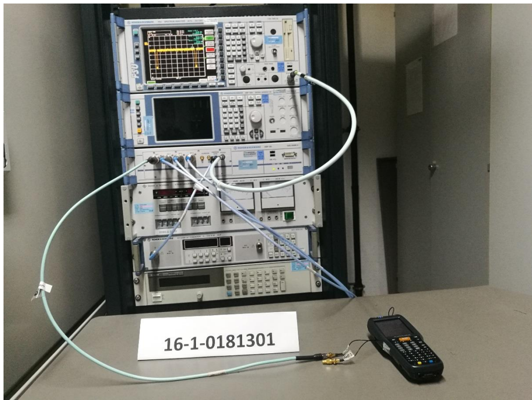
Photograph 1: Set Up 2-Overall View- ANT1 Used + ANT2 Terminated with 50 \Omega [WLAN b/g Modes]
