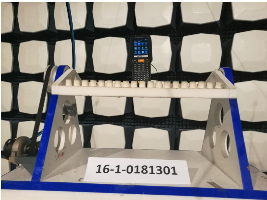
Photograph 21: Set Up 1-Close View - above 1 GHz - EUT Standing 0°- Front Side
