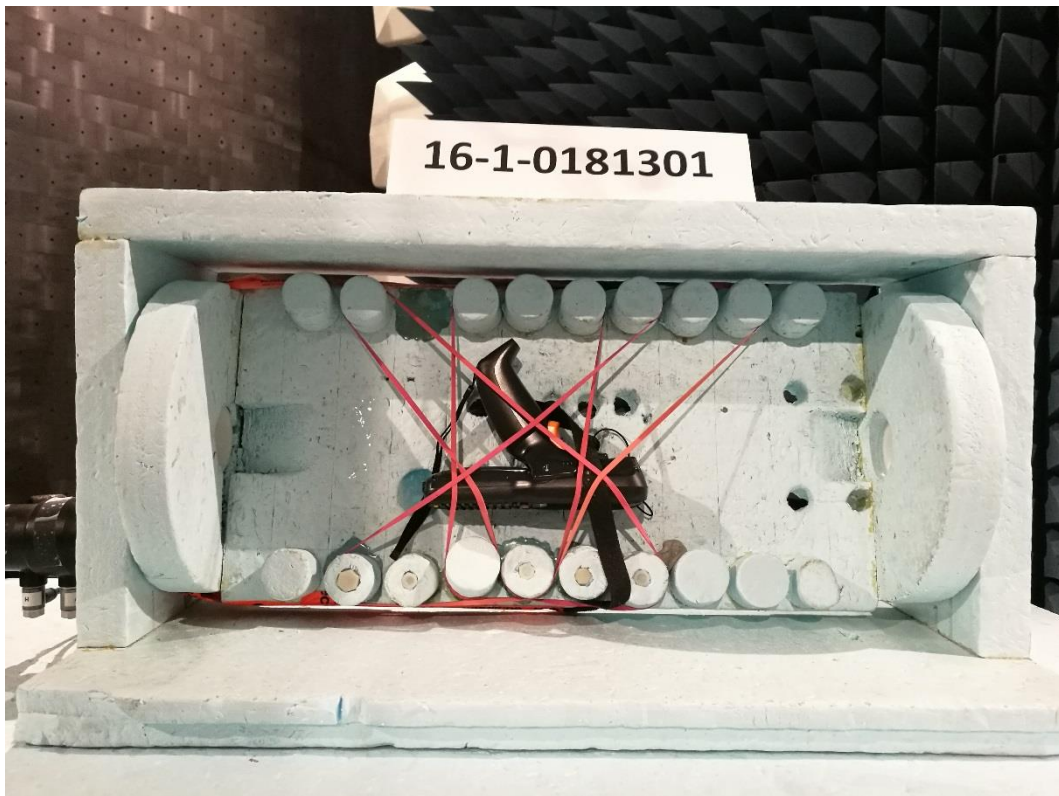
Photograph 12: Set Up 1-Close View -9 kHz-30 MHz- EUT Laying 90°- Front Side
