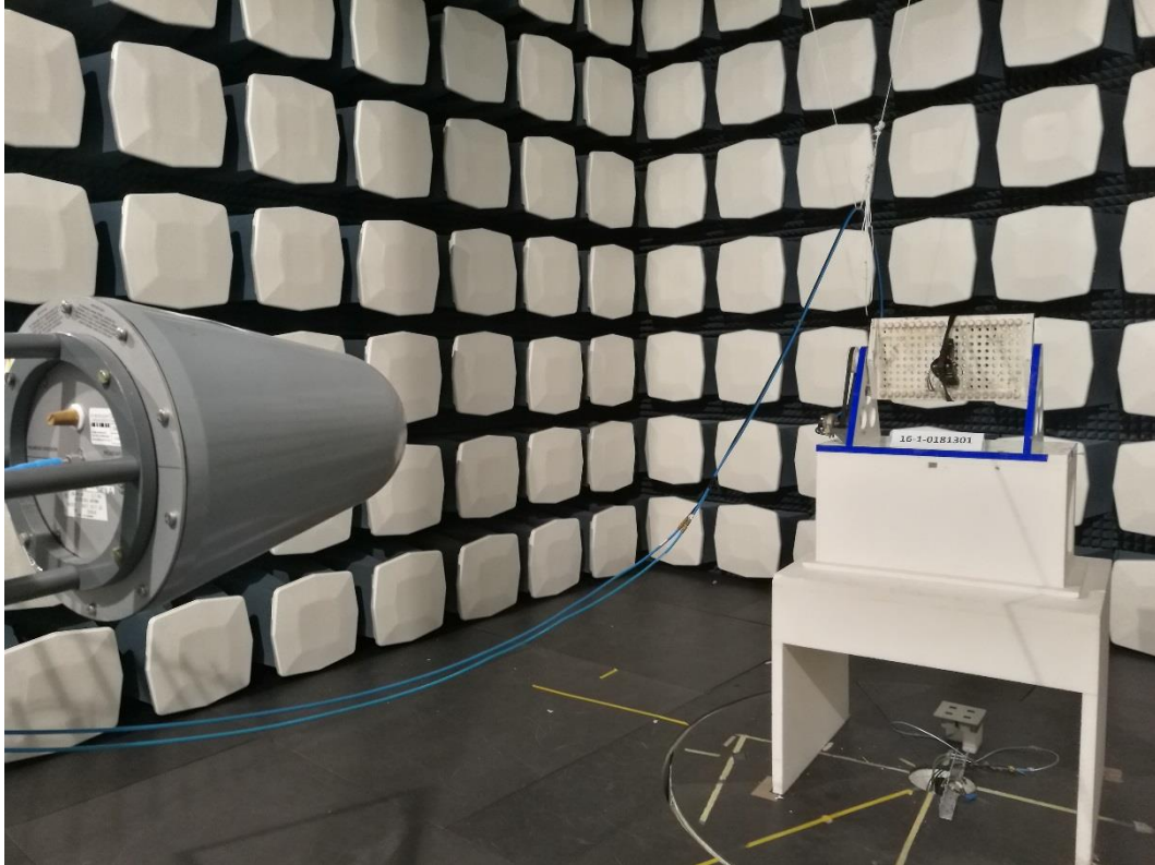
Photograph 18: Set Up 1-Overall View - above 1 GHz- EUT Standing 90° - Front Side
