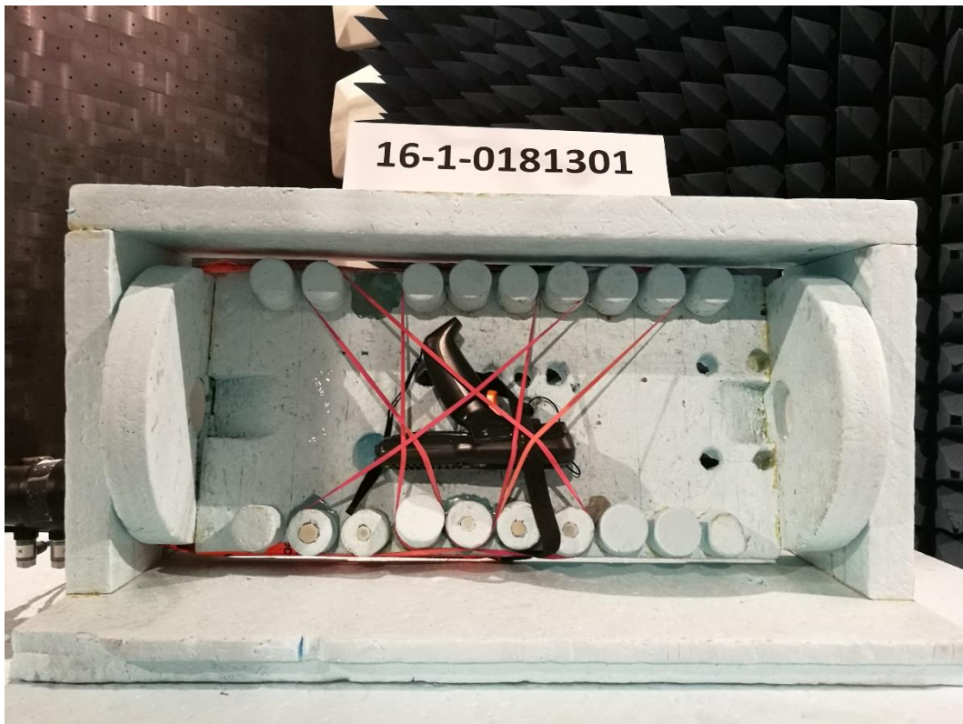
Photograph 16: Set Up 1-Close View - 30 MHz-1 GHz - EUT Laying 90°- Front Side
