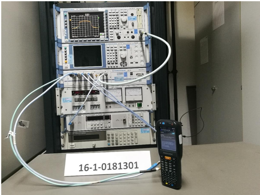
Photograph 8: Set Up 2-Overall View- ANT1 + ANT2 used [WLAN n Mode-MIMO]
