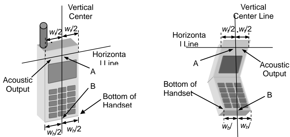
Fig-4.1 Illustration for Handset Vertical and Horizontal Reference Lines
