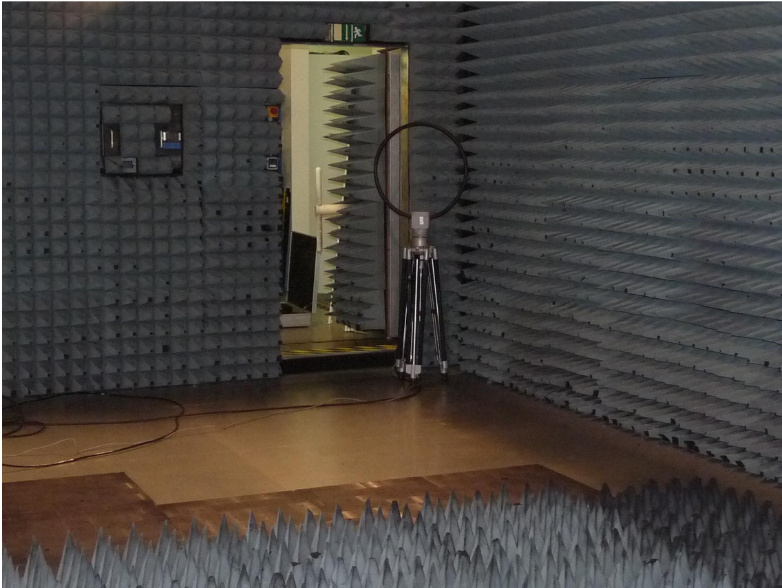
Photo 1: Radiated test setup for H-Field
