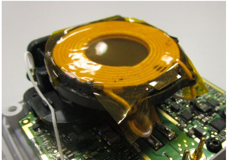
WPT Rx Coil assembly
