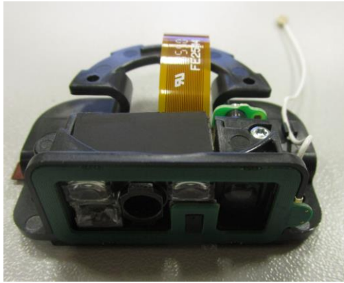
Reader Assembly
