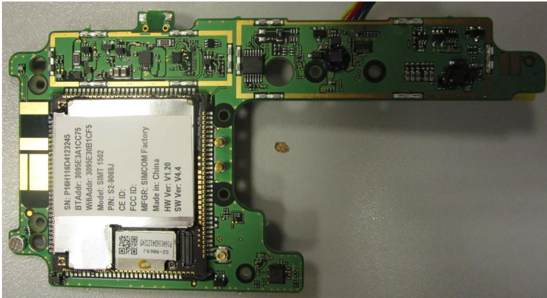
Mainboard (Bottom)
