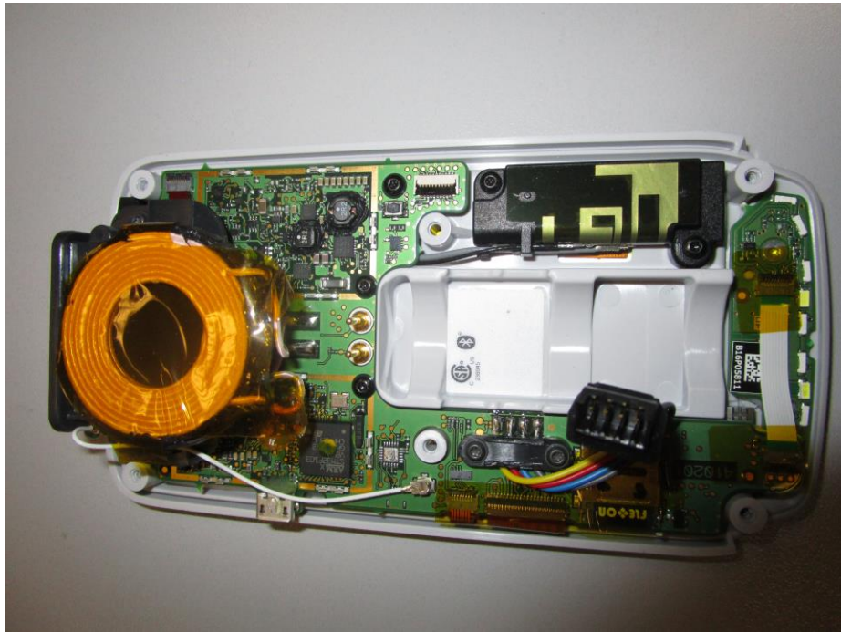
Internal Overview
