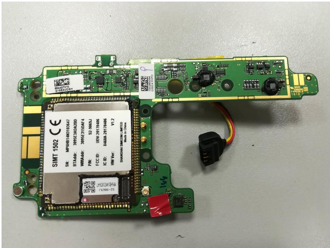
Mainboard (Bottom)
