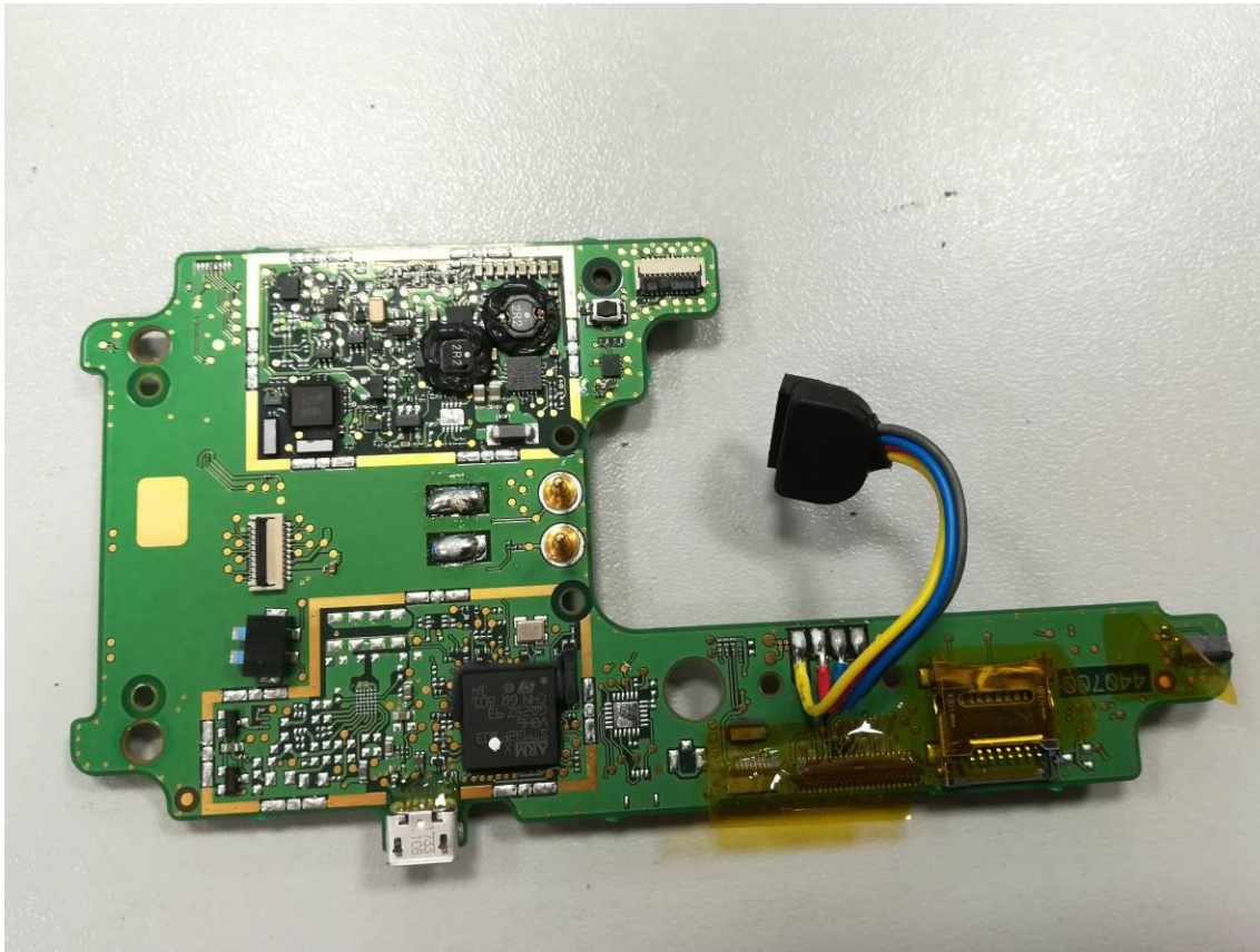
Mainboard (Top)
