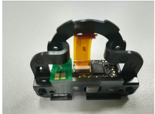
Reader Assembly
