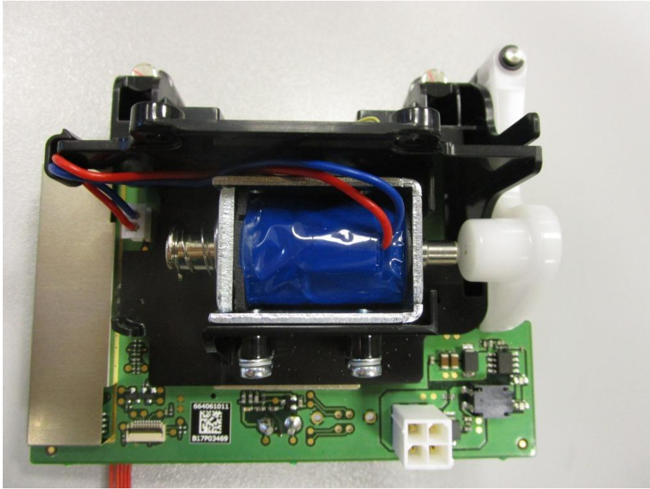
Internal Assembly
