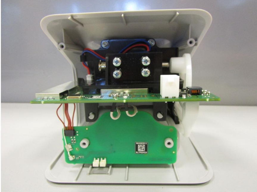
Internal Overview (1)
