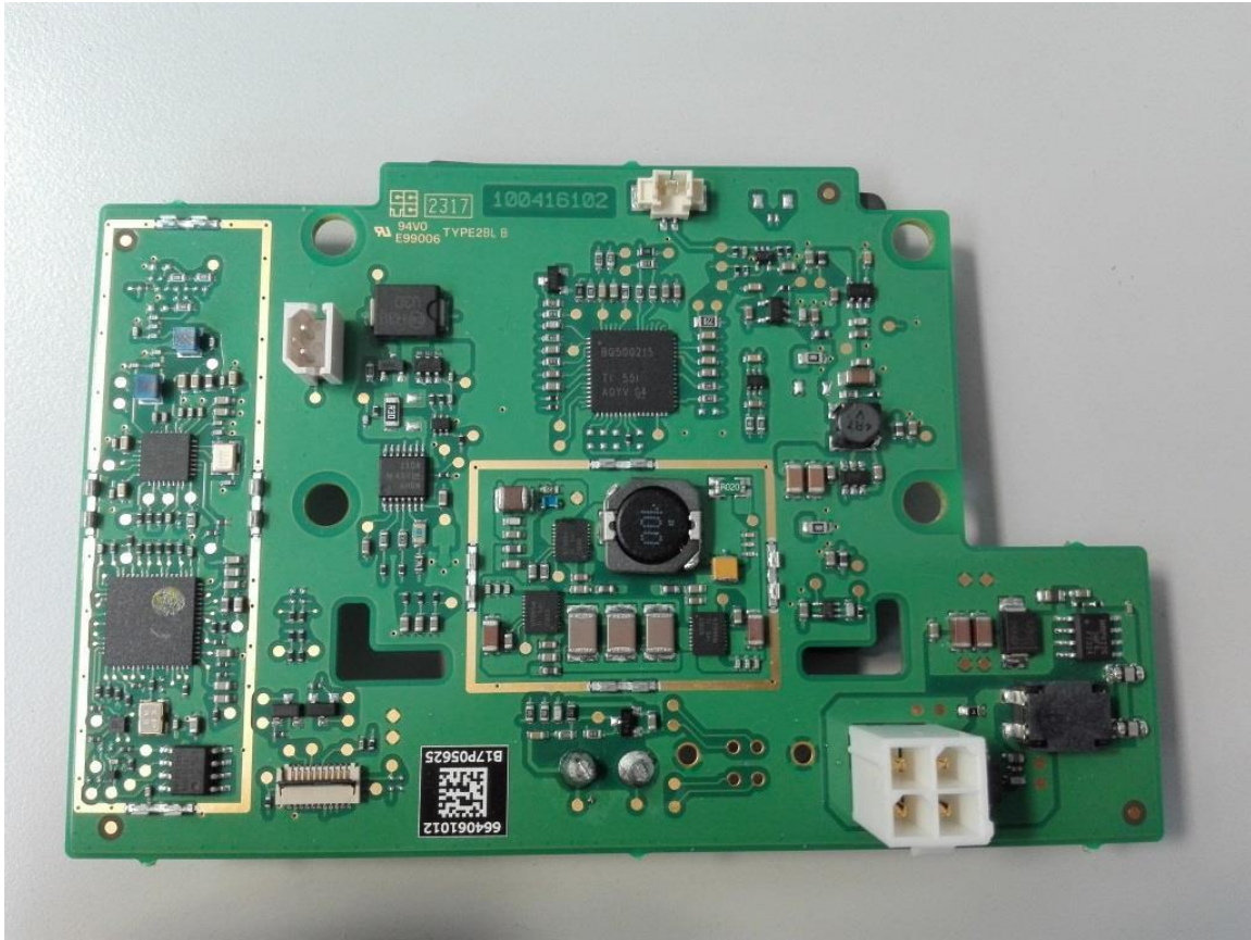
Main board (with metal shields removed)
