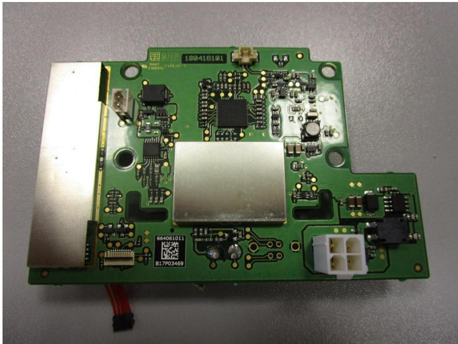
Main board (with metal shields)
