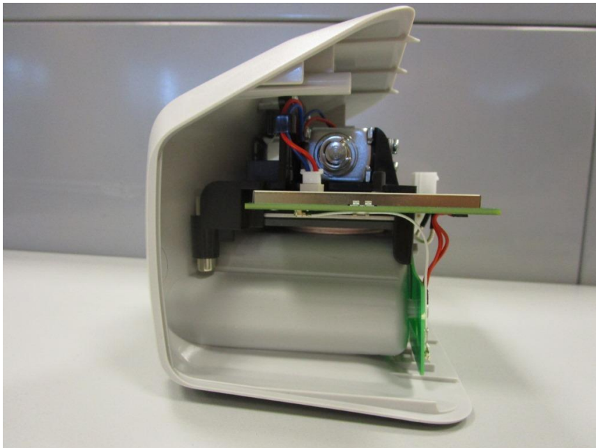
Internal Overview (2)
