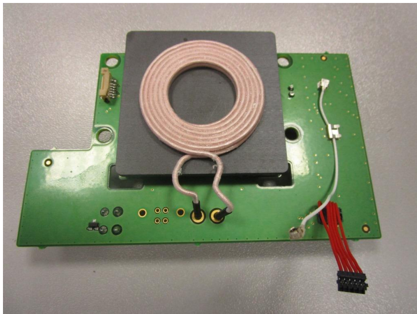
Main board (WPT coil antenna side)
