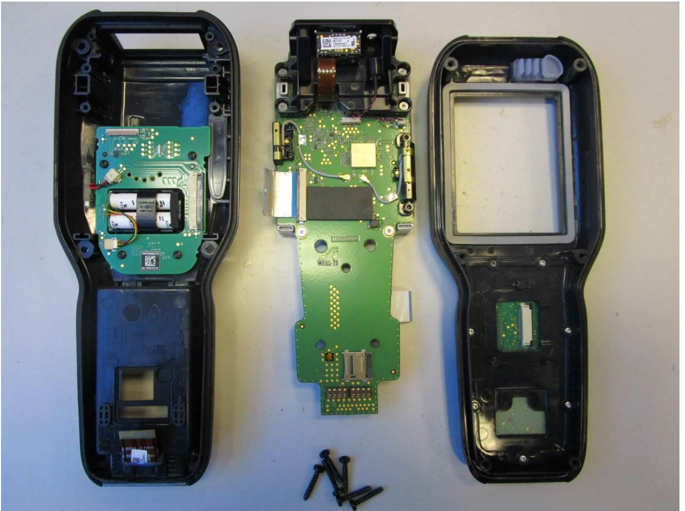
Internal Overview - bottom
