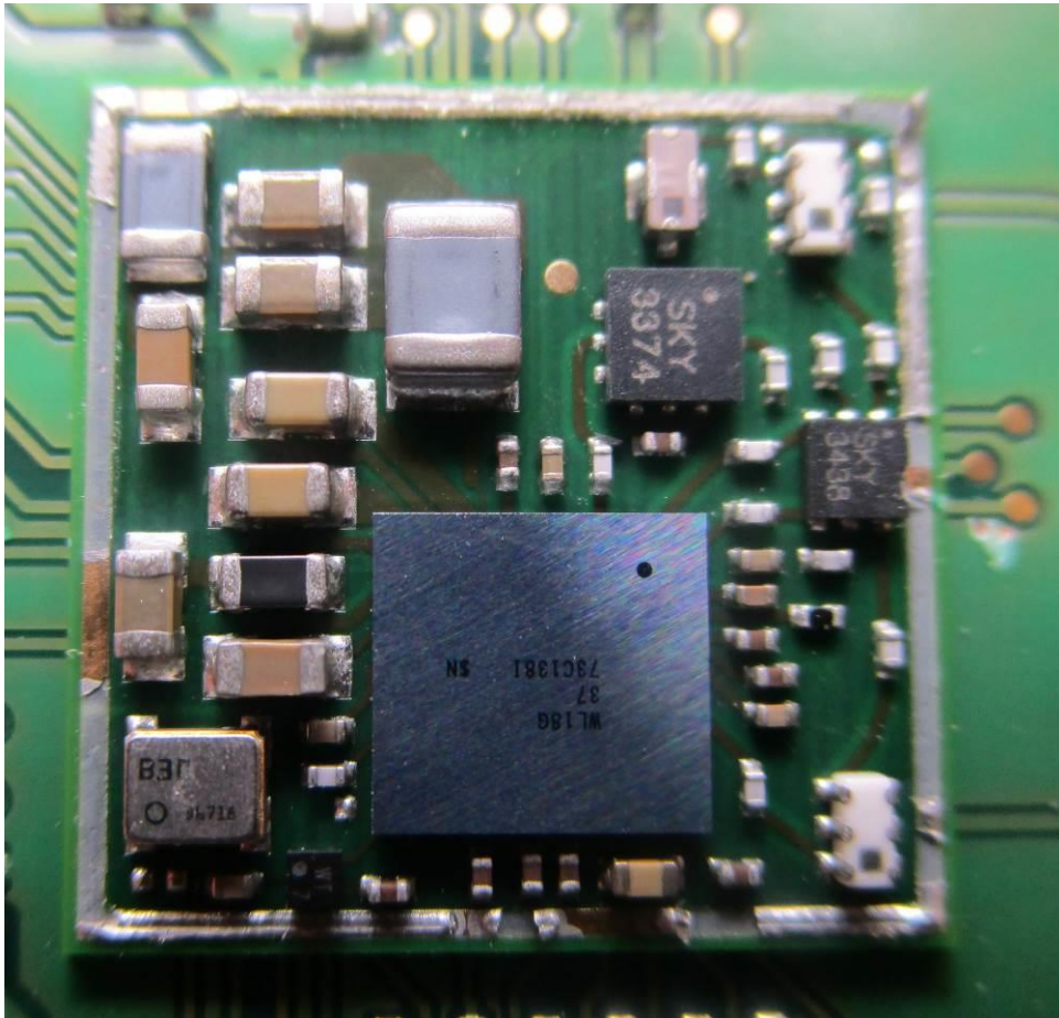
WLAN+BT radio module (internal view)
