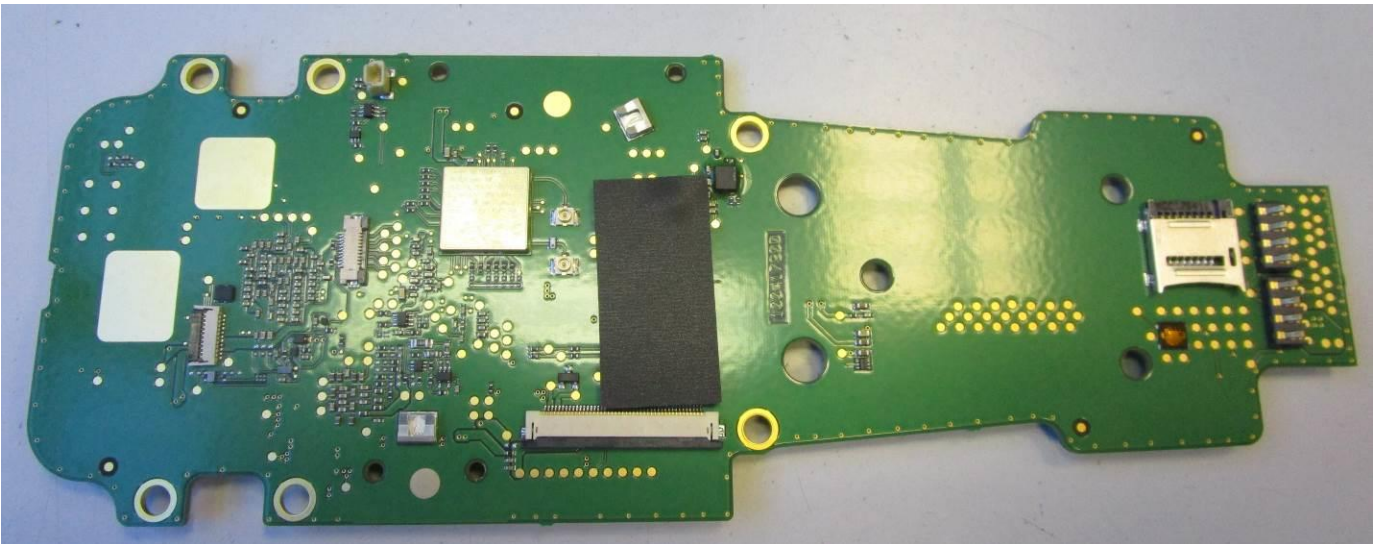
Mainboard
