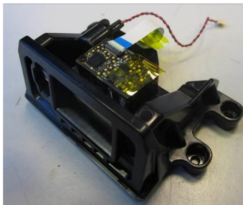
1D Imager with plastic support and Green Spot
