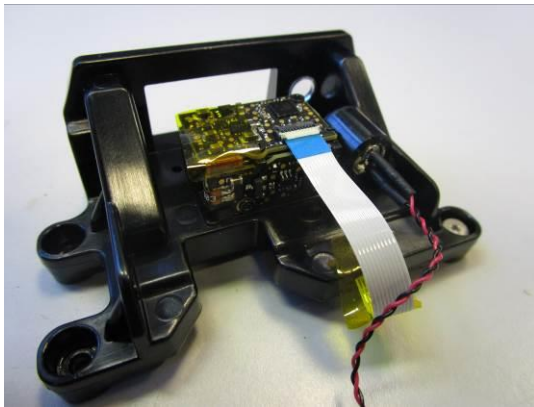
1D Imager with plastic support and Green Spot
