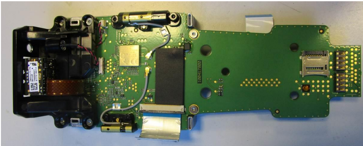
Internal Assembly
