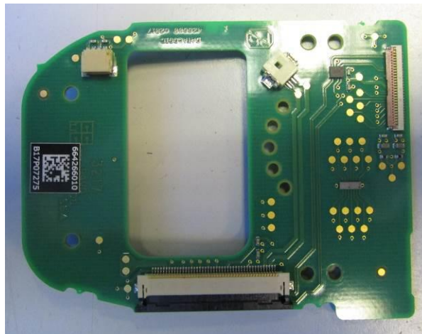
Photograph 16: FALCON X4 –Trigger Board Front Side
