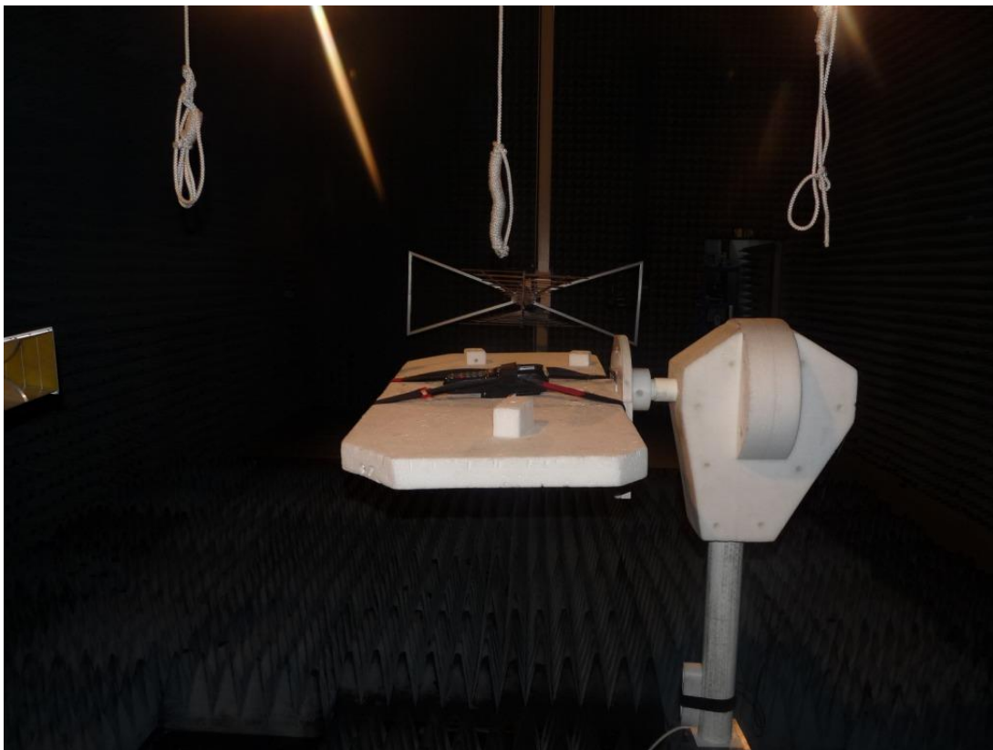
Photo 3: Test setup for FCC 15.247 and FCC 15.407
