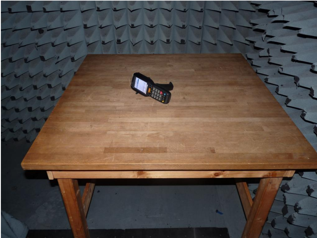
Photo 2: Test setup for FCC 15.247 and FCC 15.407
