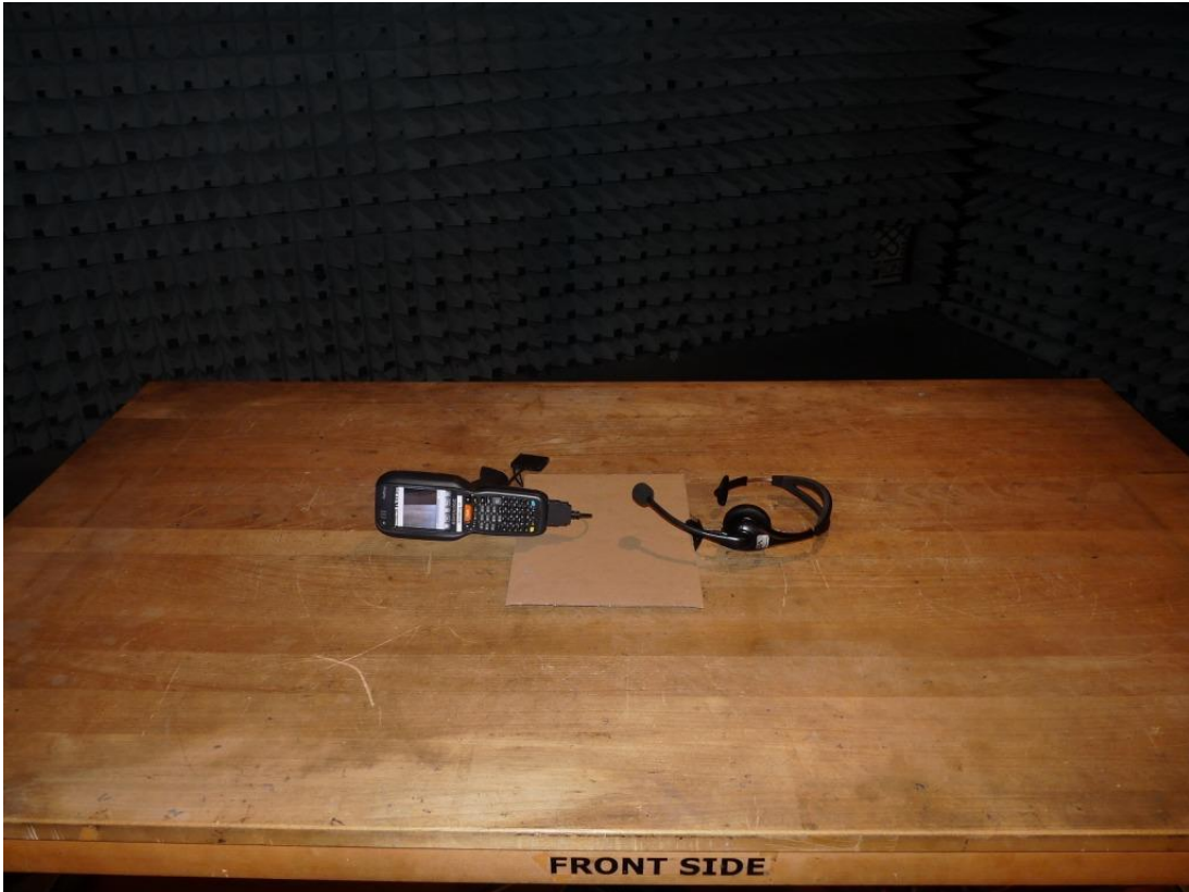
Photo 3: Test setup for radiated measurements (unintentional radiator §15); Setup AJ01
