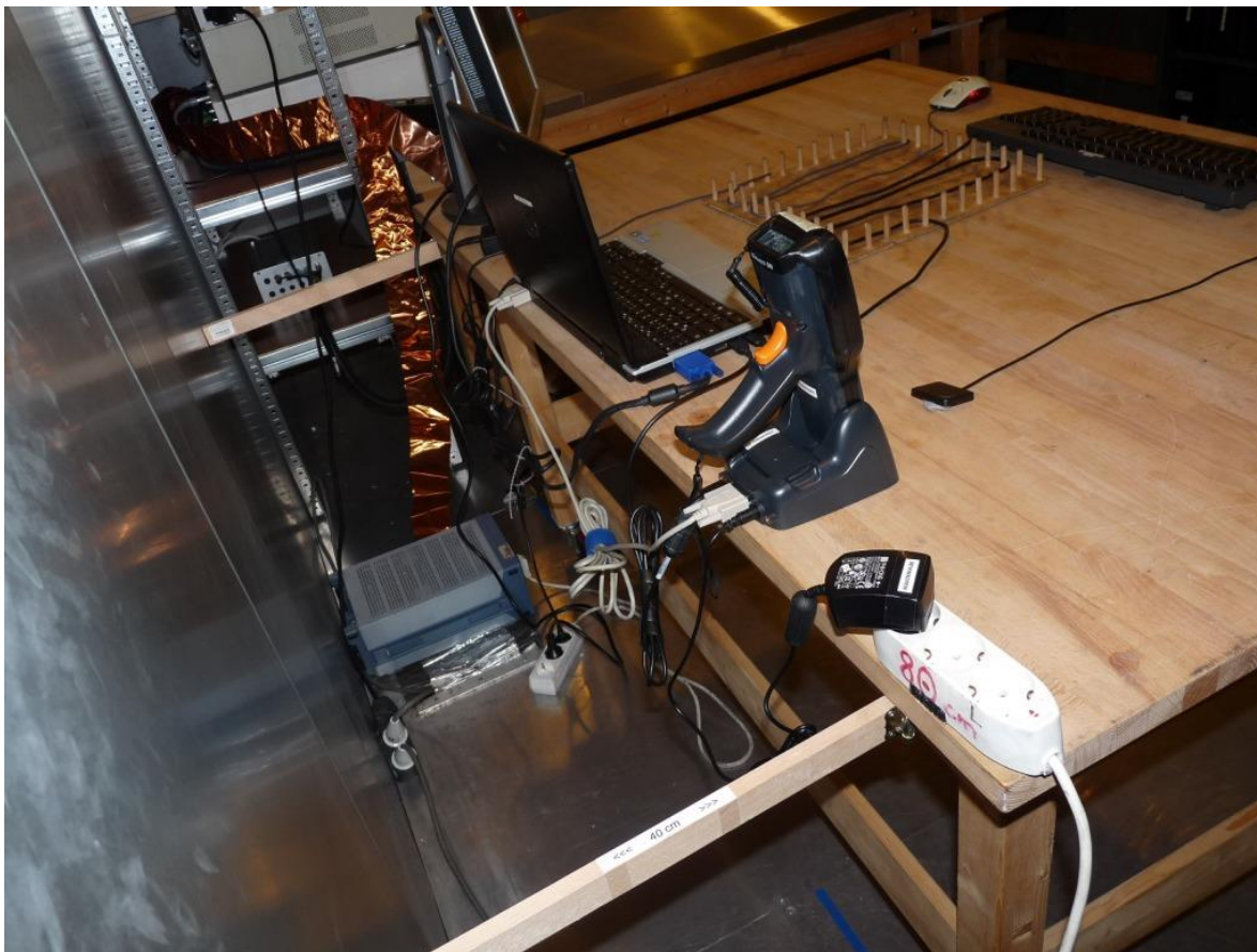
Photo 2: Test setup for conducted measurements (AC Port (power line), unintentional radiator §15)
