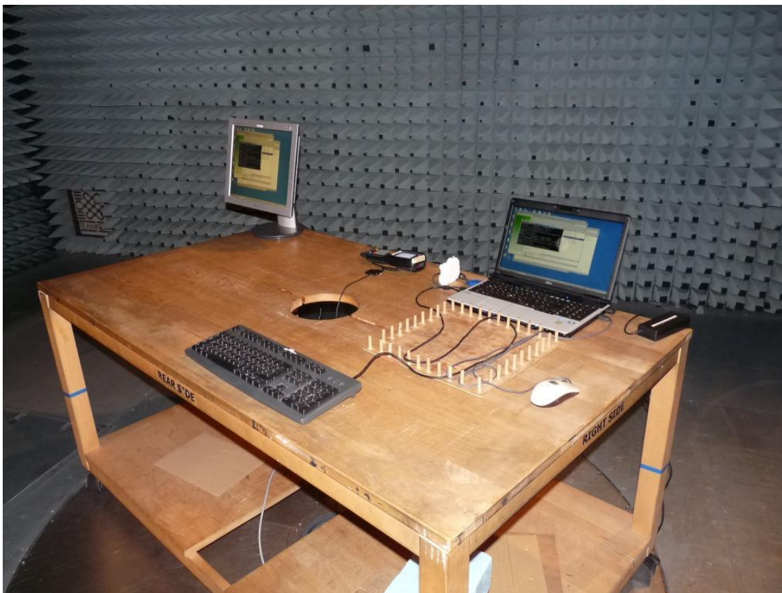
Photo 7: Test setup for radiated measurements (unintentional radiator §15), front view, Setup AF01
