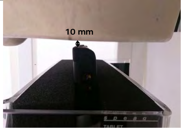
Fig.12 EUT Left side to flat phantom
