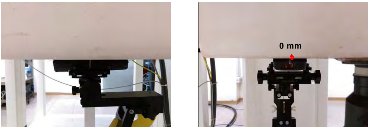
Fig.11 EUT Front side to flat phantom
