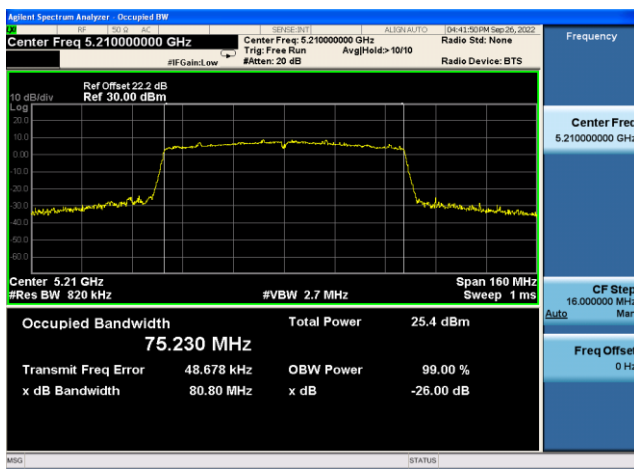
Channel 42 (5210MHz)
