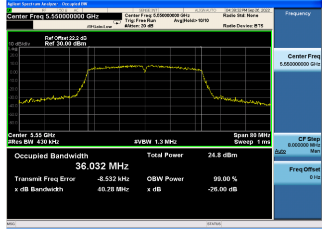
Channel 110 (5550MHz)
