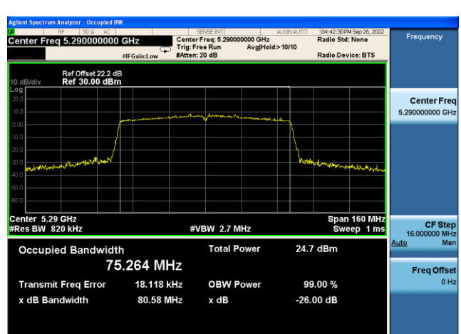
Channel 58 (5290MHz)
