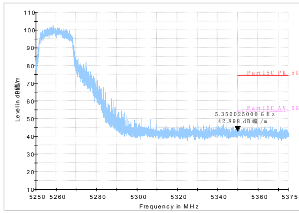
Peak detector
