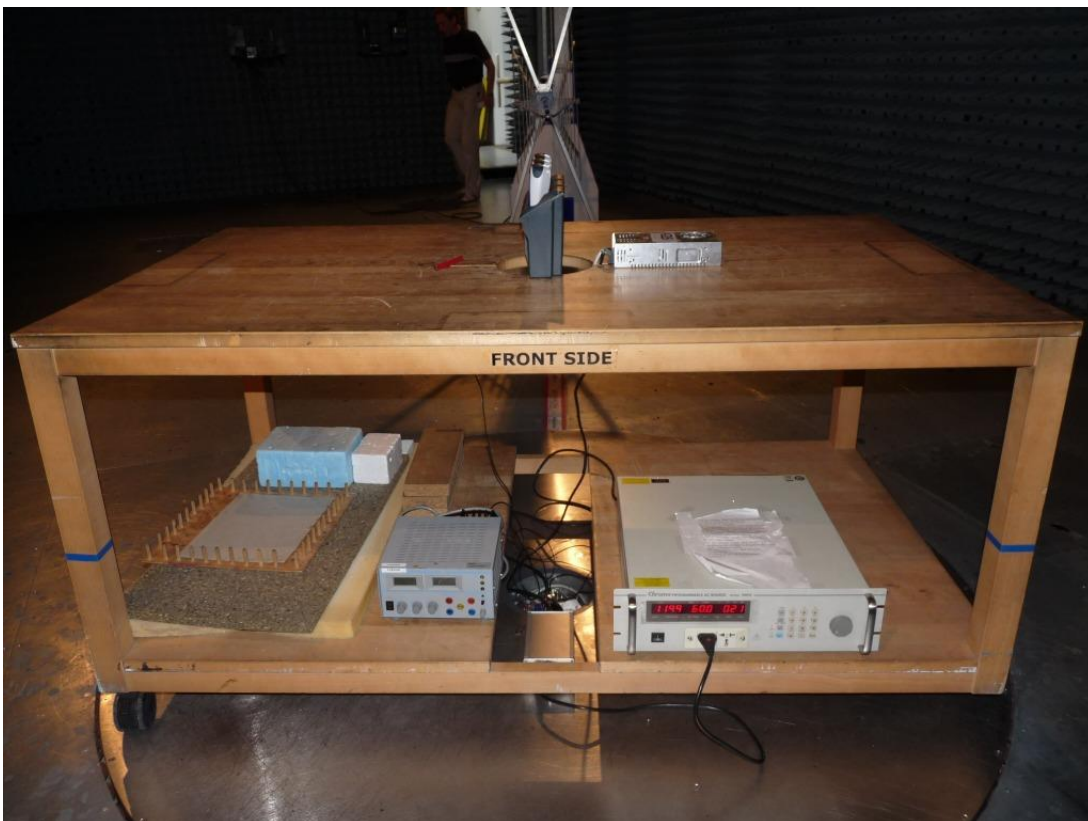
Photo 4: Test setup for radiated measurements, computer peripheral setup, EUT connected via USB cable to computer, intentional/ unintentional radiator §15.
