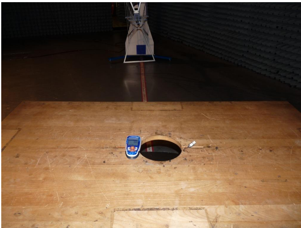
Photo 3: Test setup in semi anechoic chamber
