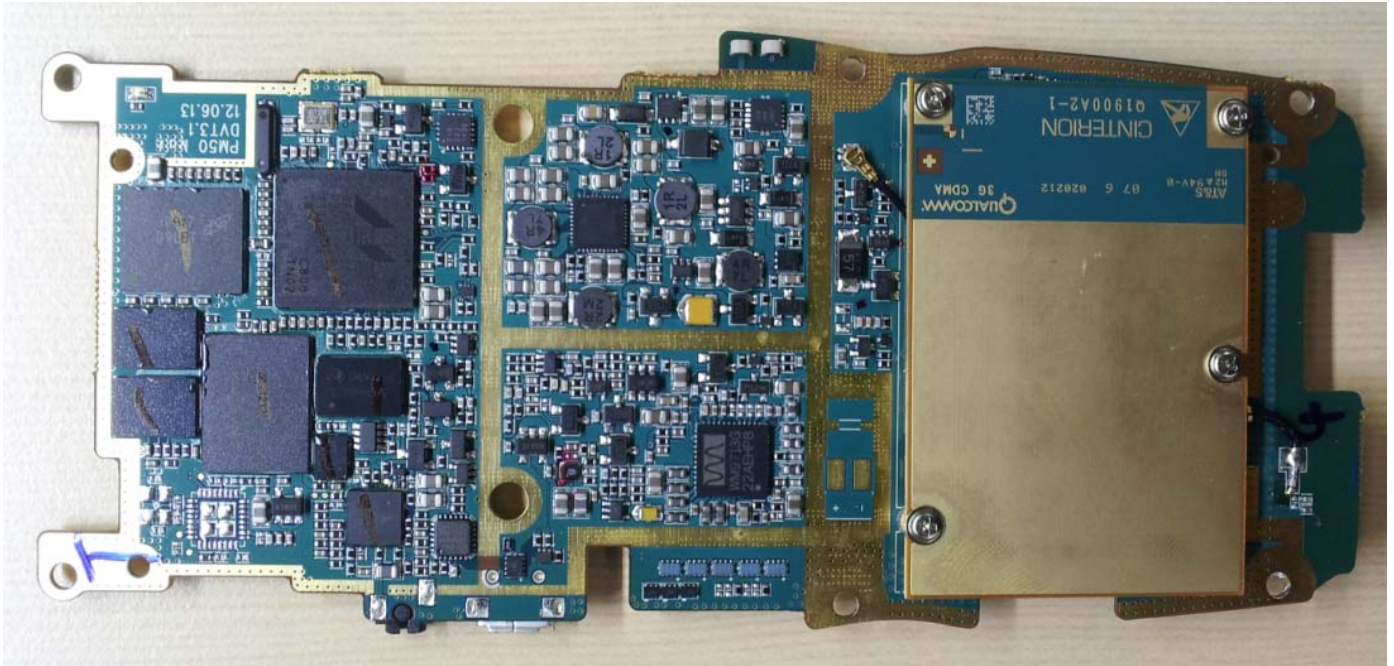
< Main PCB Front Side >
