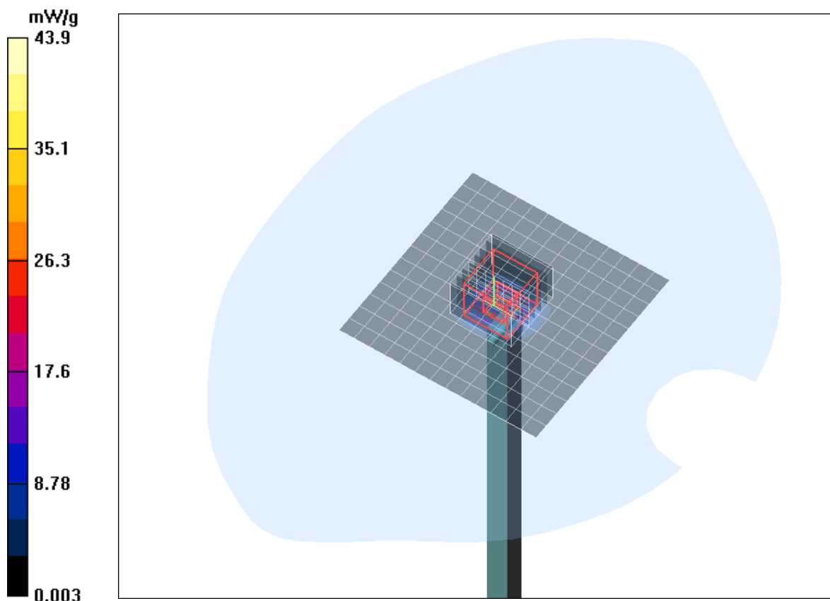
Fig. 15: Validation measurement 5800 MHz Head (May 21, 2012), coarse grid. Ambient Temperature: 21.8° C, Liquid Temperature: 21.5° C.
