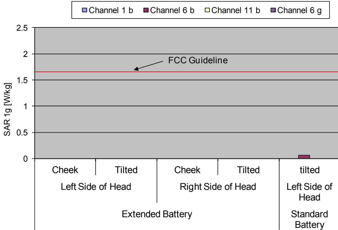
Fig. 8: The measured head SAR values for the Datalogic SKORPIO X3 for IEEE 802.11 b/g in head configuration, in comparison to the FCC exposure limit.
