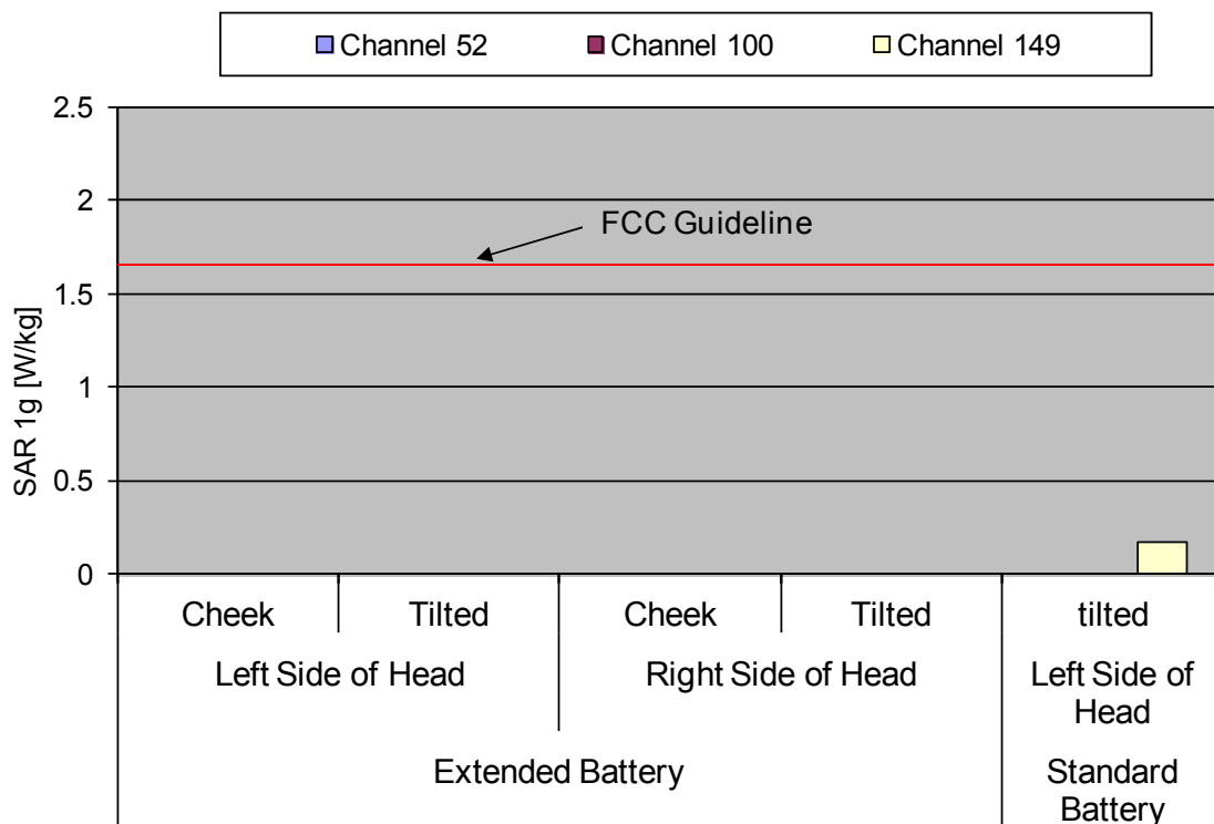
Fig. 10: The measured head SAR values for the Datalogic SKORPIO X3 for IEEE 802.11 a in head configuration, in comparison to the FCC exposure limit.
