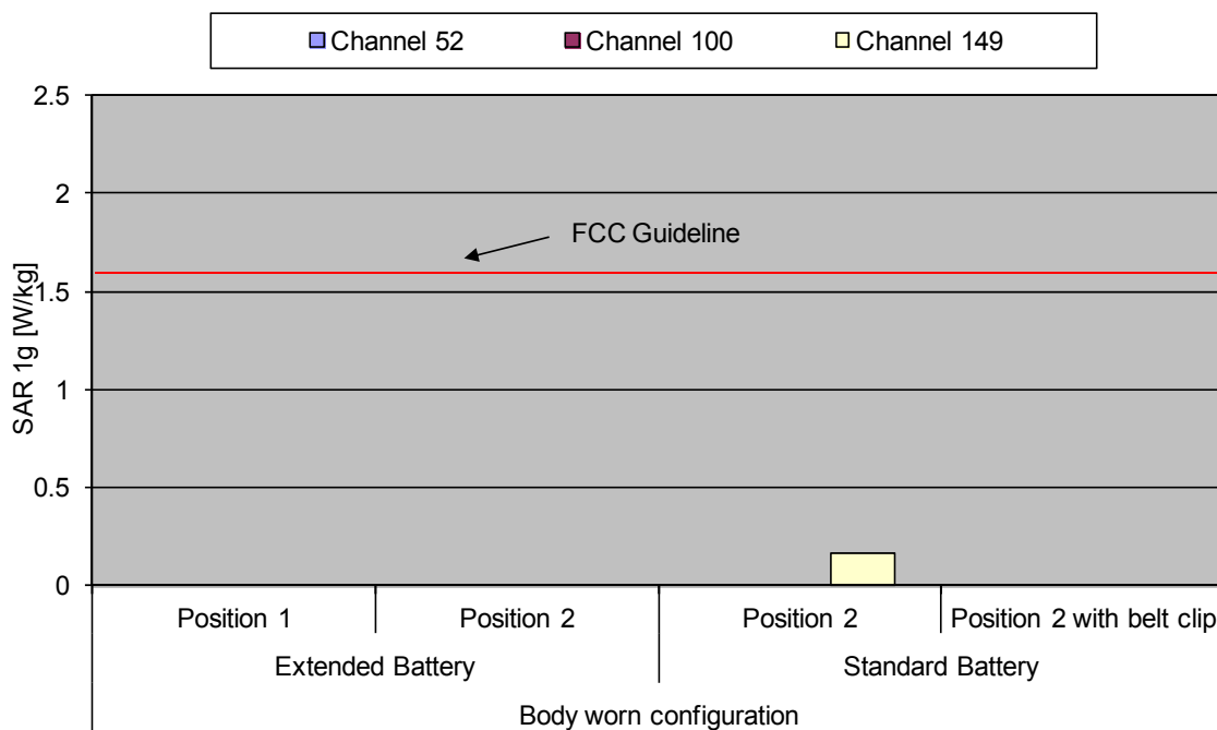
Fig. 11: The measured body SAR values for the Datalogic SKORPIO X3 for IEEE 802.11 a in body worn configuration, in comparison to the FCC exposure limit.
