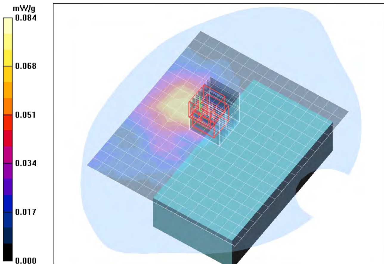
Fig. 79: SAR distribution for IEEE 802.11 a, channel 124, body worn configuration, display towards the phantom, 15 mm distance (May 18, 2010; Ambient Temperature: 21.9° C; Liquid Temperature: 21.3° C).
