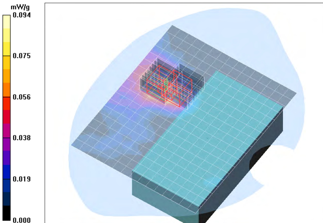
Fig. 92: SAR distribution for IEEE 802.11 a, channel 161, body worn configuration, display towards the phantom, 15 mm distance (May 14, 2010; Ambient Temperature: 21.8° C; Liquid Temperature: 21.2° C).
