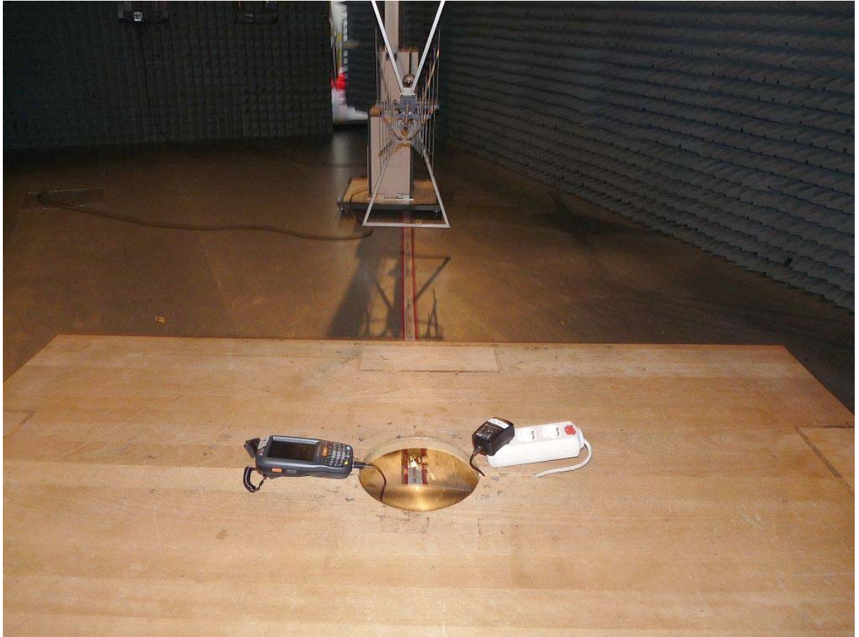
setup for radiated tests, EUT + AC/DC adapter
