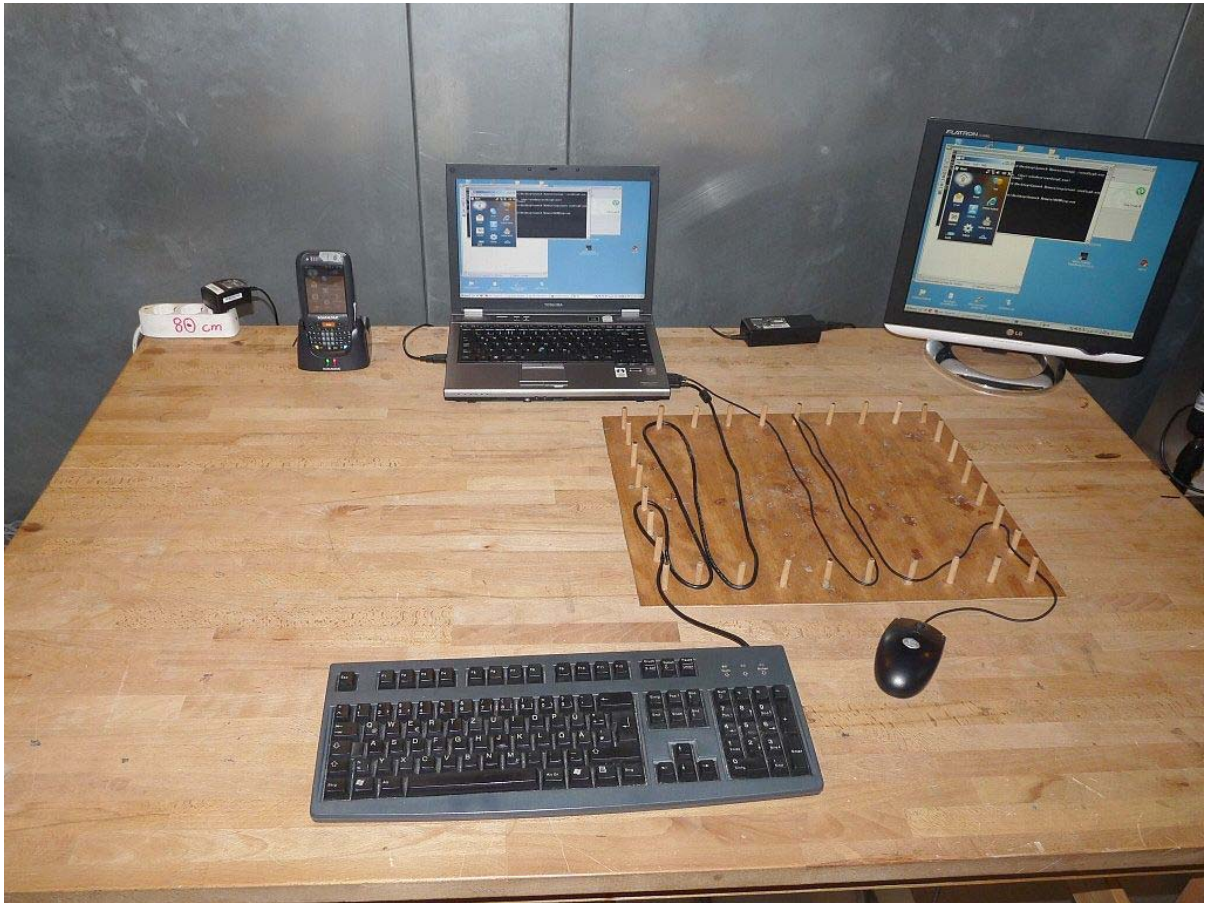
setup for conducted tests, EUT + Cradle + AC/DC adapter (of cradle); USB + RS232 connection to Laptop
