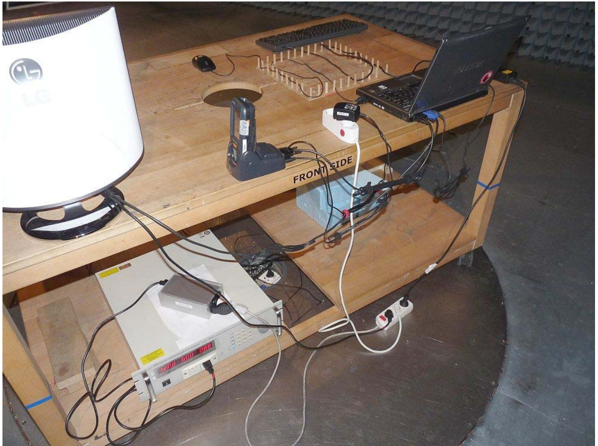
setup for radiated tests, EUT + Cradle + AC/DC adapter (of cradle); USB + RS232 connection to Laptop
