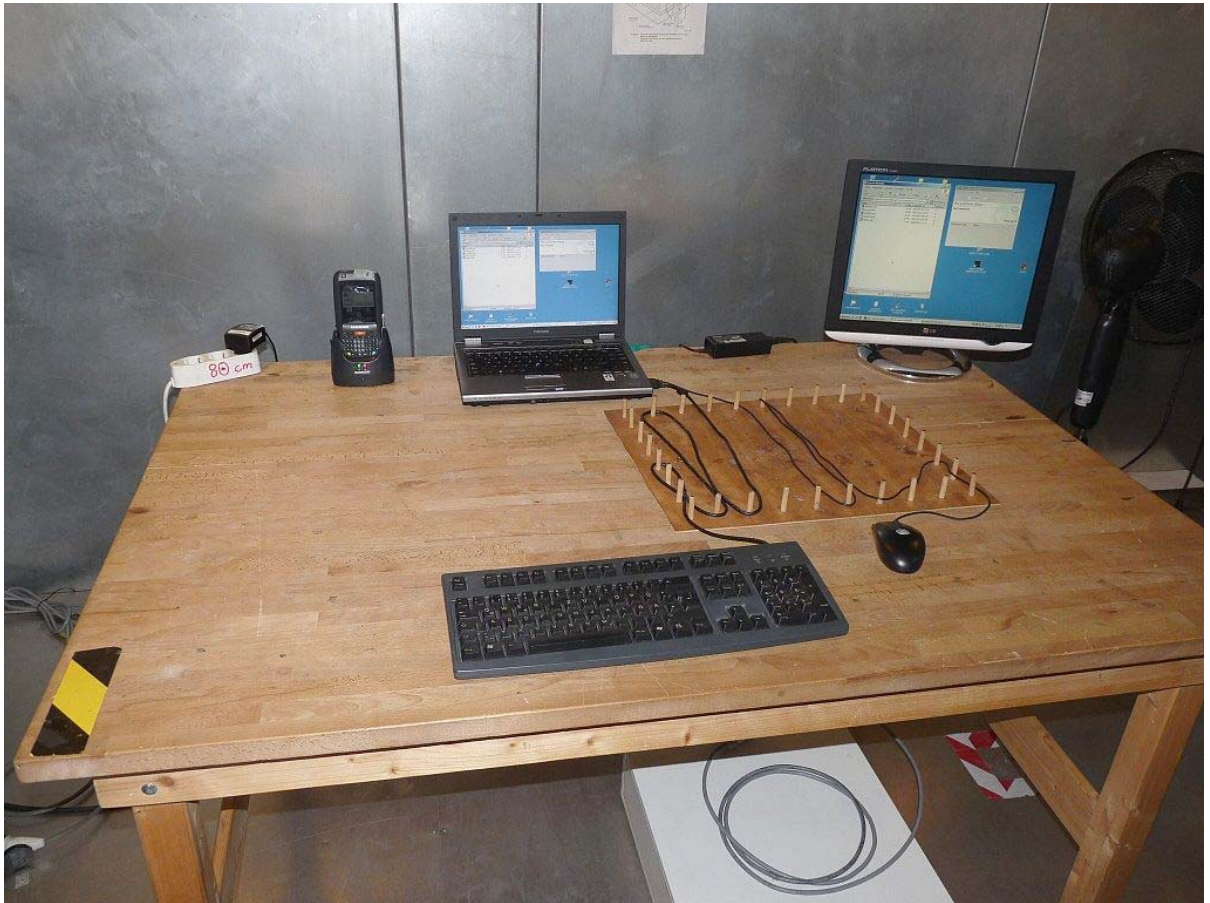
setup for conducted tests, EUT + Cradle + AC/DC adapter (of cradle); LAN connection to Laptop
