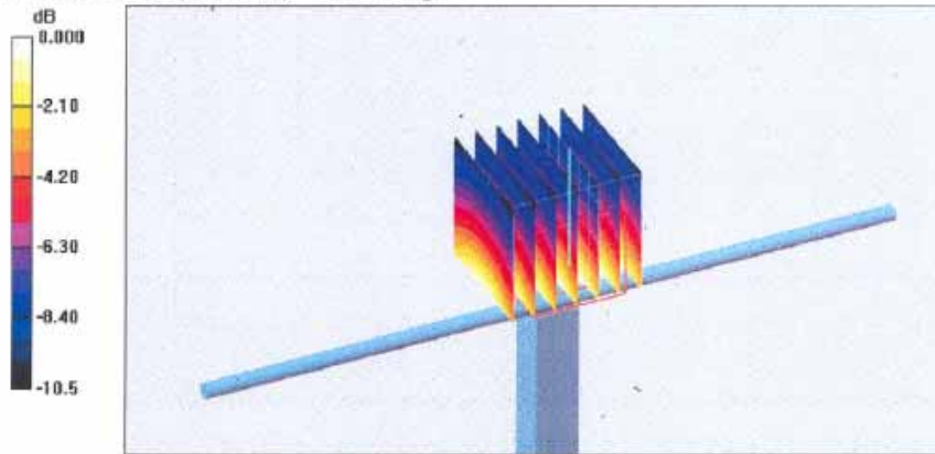
0 dB = 2.58mW/g
