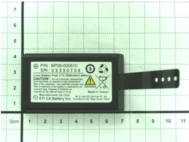
Battery 1_Front
