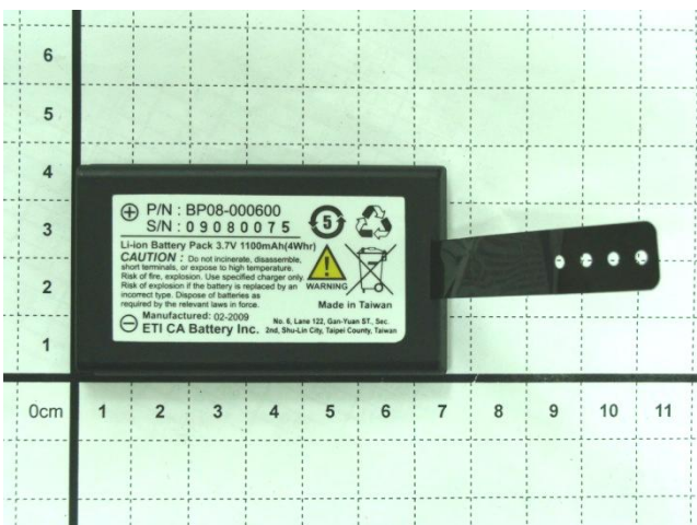
Battery 2_Front
