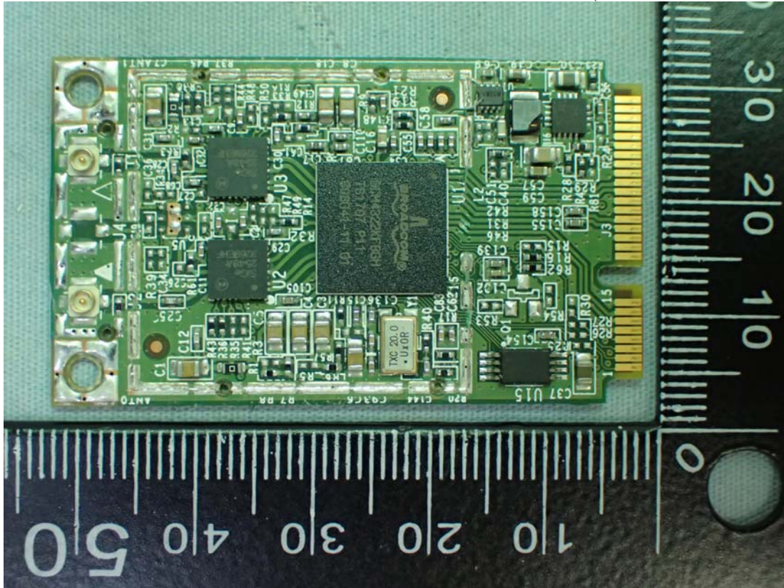
Figure 9 Internal View (Removed Shielded Cover)
