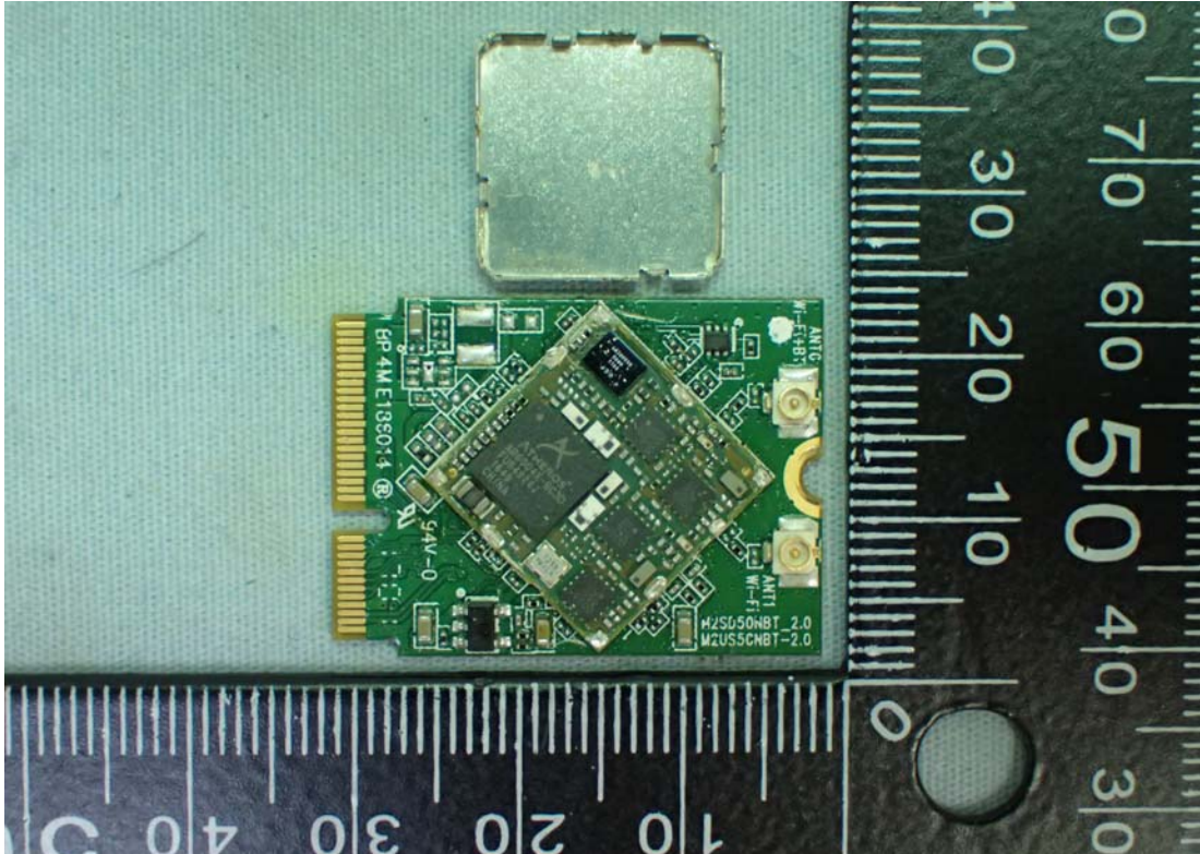
Figure 9 Internal View (Removed Shielded Cover)
