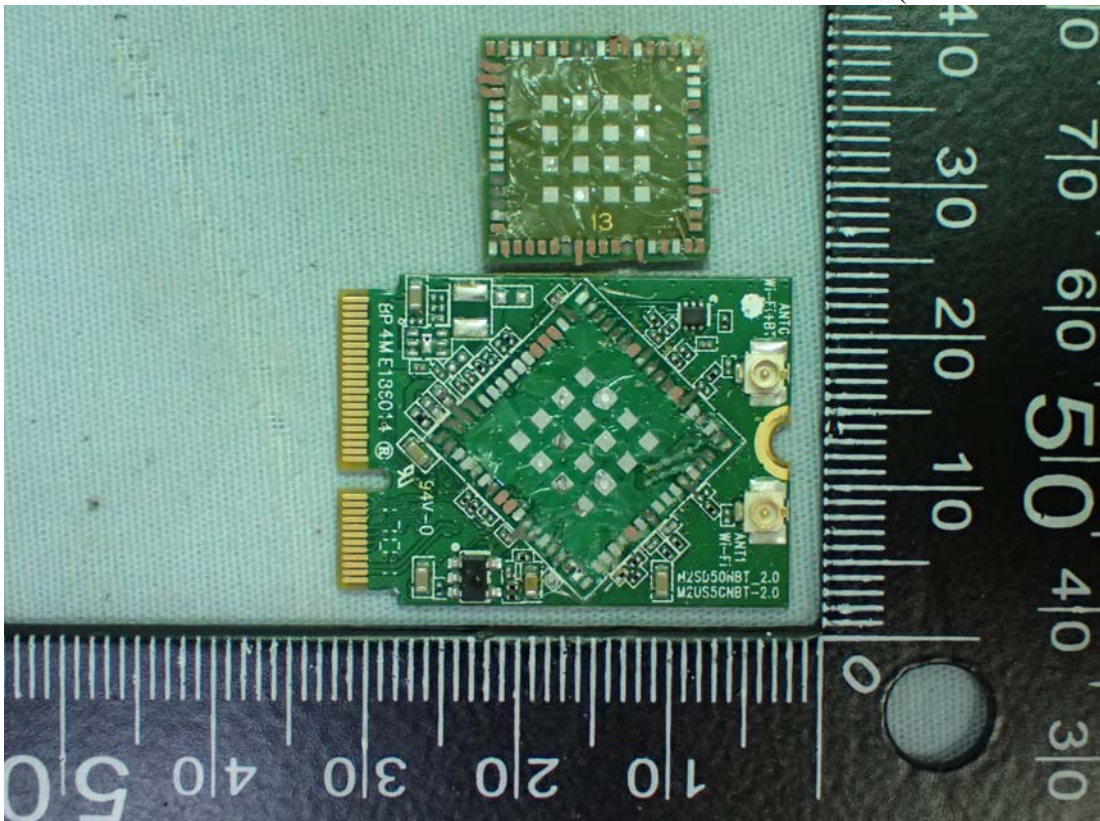
Figure 10 Internal View (Removed RF Board)
