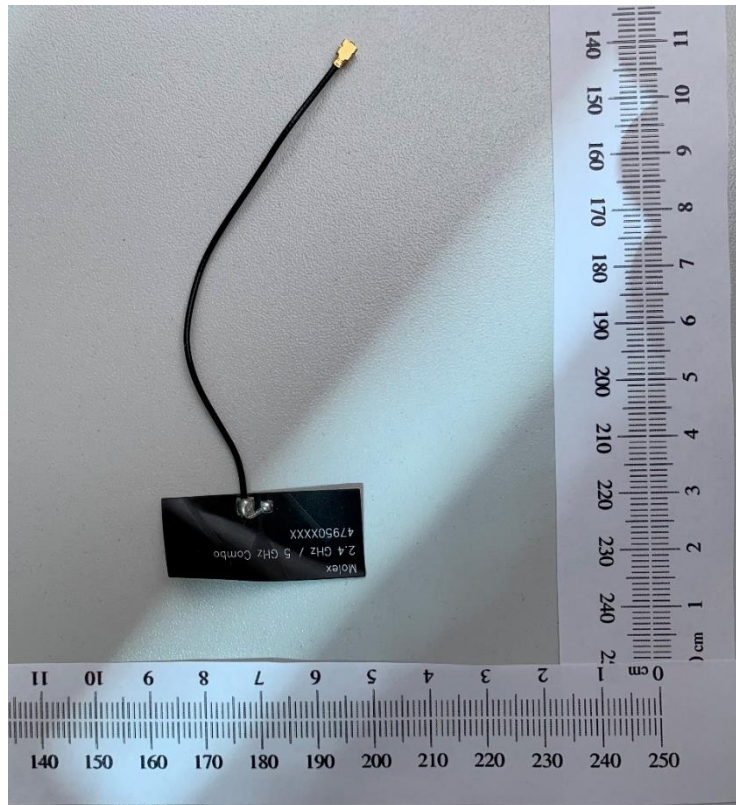
Bluetooth Antenna
