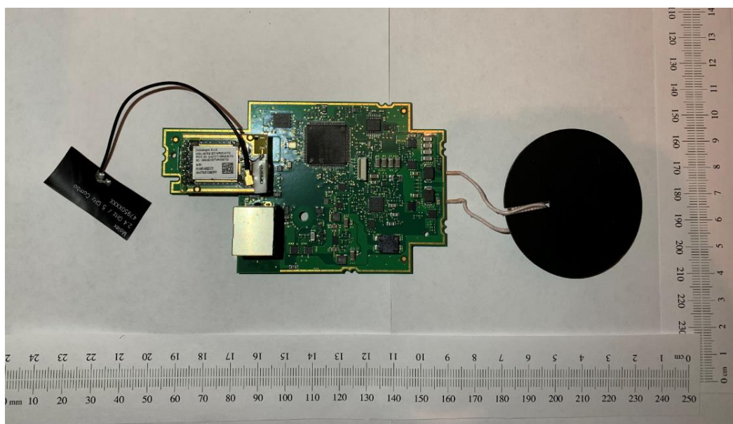
Internal assembly of WLC4190 Bluetooth version
