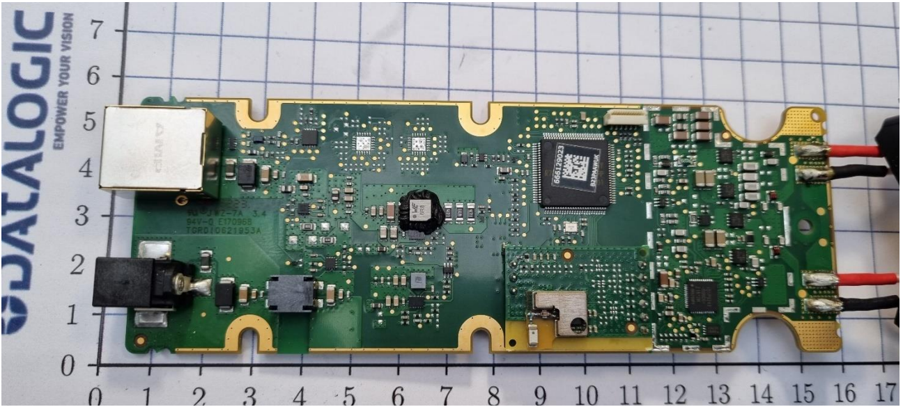
Motherboard bottom side - 2
