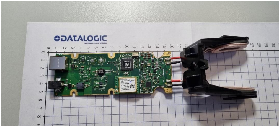
Motherboard bottom side - 2
