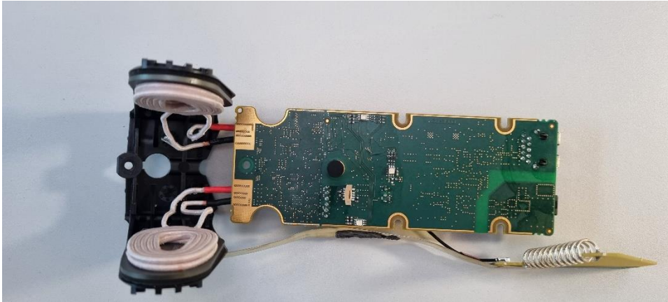
Motherboard upper side
