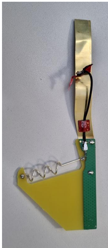
910 MHz Antenna
