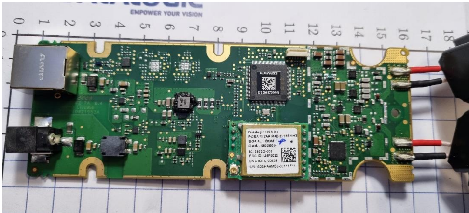
Motherboard bottom side - 3
