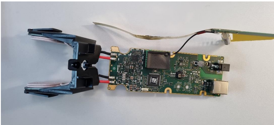
Motherboard bottom side - 1
