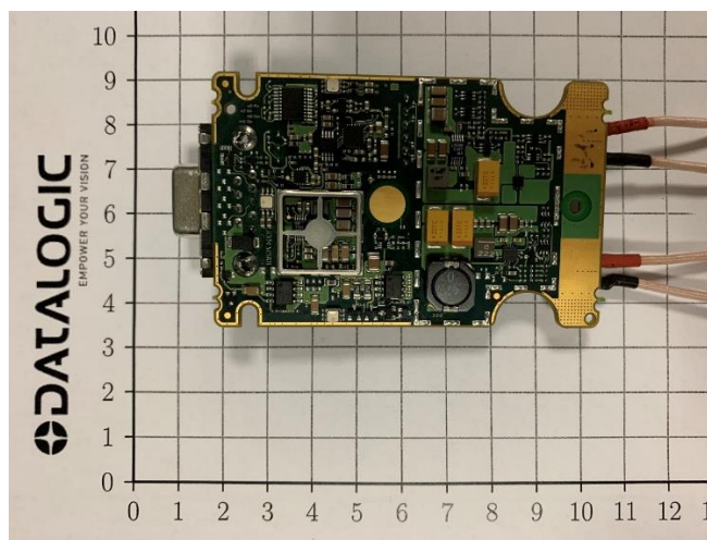
Main Board Side 1
