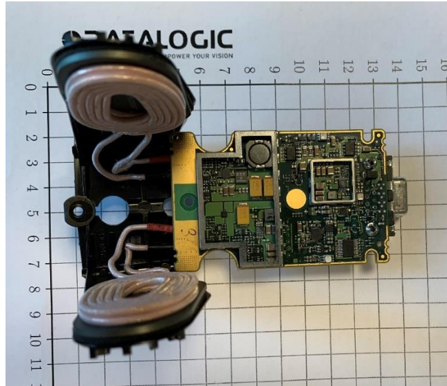
Internal assembly of BC9600-910
