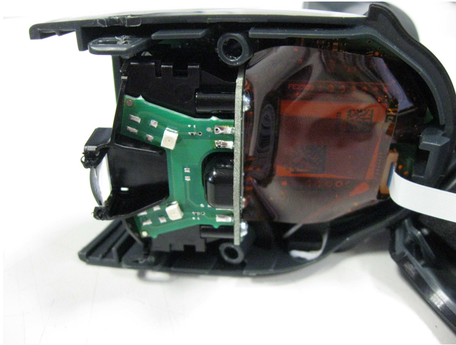
Fig. 1: internal boards
