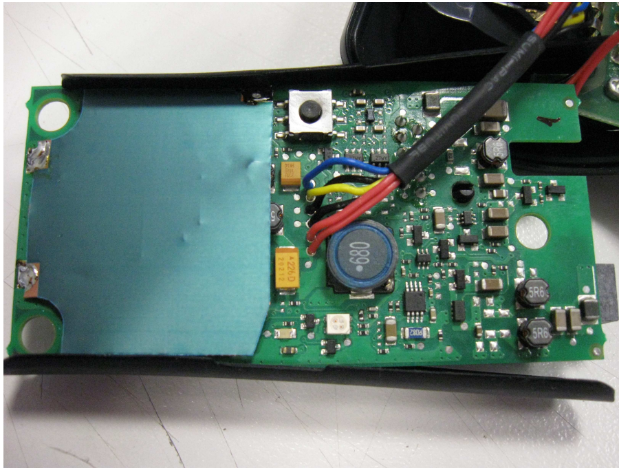
Fig. 5: particular of the electronic board
