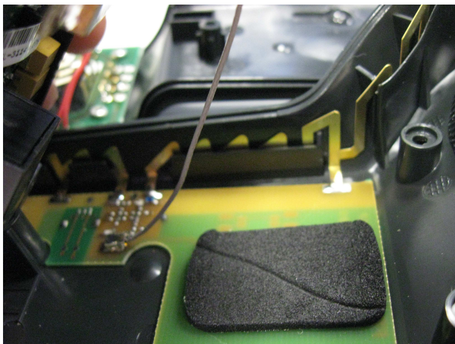
Fig. 3: particular of the antenna
