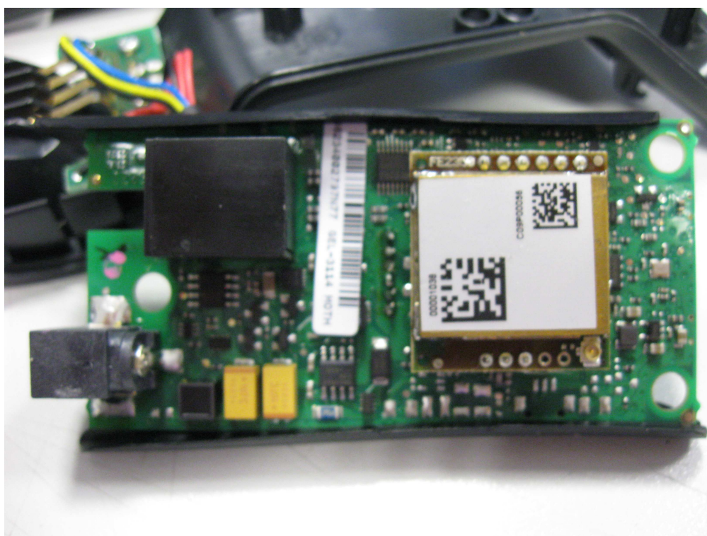
Fig. 4: particular of the radio module
