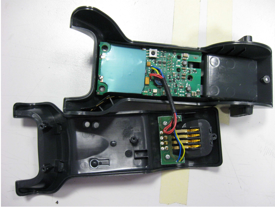
Fig. 1: internal boards
