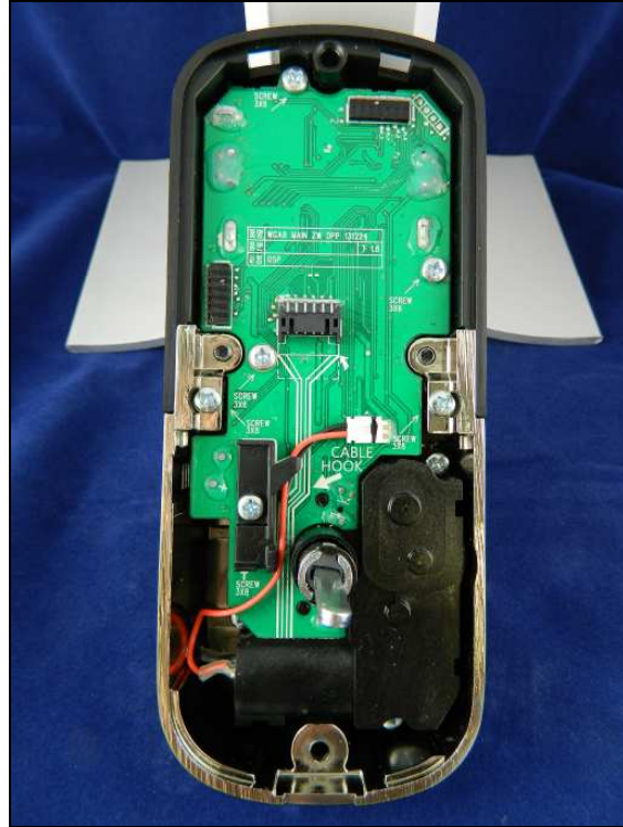
Figure 7: Internal Photo – YRD110-ZW-US
