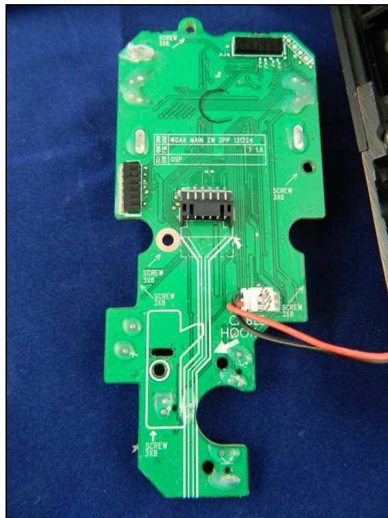
Figure 4: Internal Photo – YRD120-ZW-US
