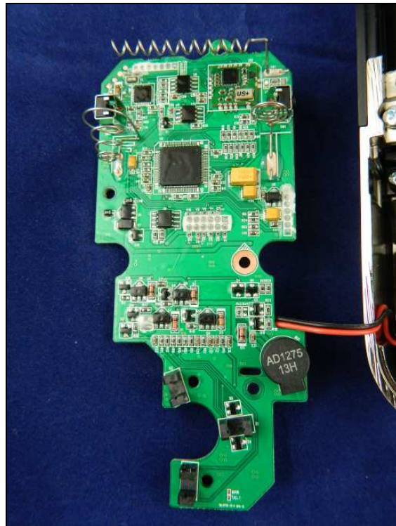
Figure 8: Internal Photo – YRD110-ZW-US
