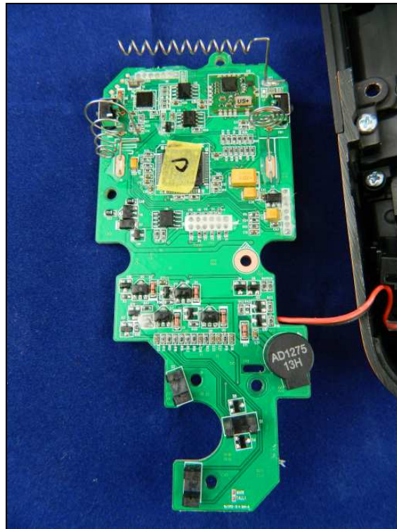
Figure 3: Internal Photo – YRD120-ZW-US
