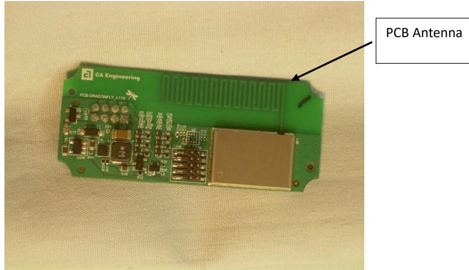
Photograph 1 – Top View of the PCB with Shield
