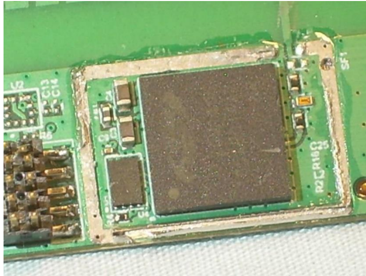
Photograph 3 – View of the Circuitry under the RF Shield
