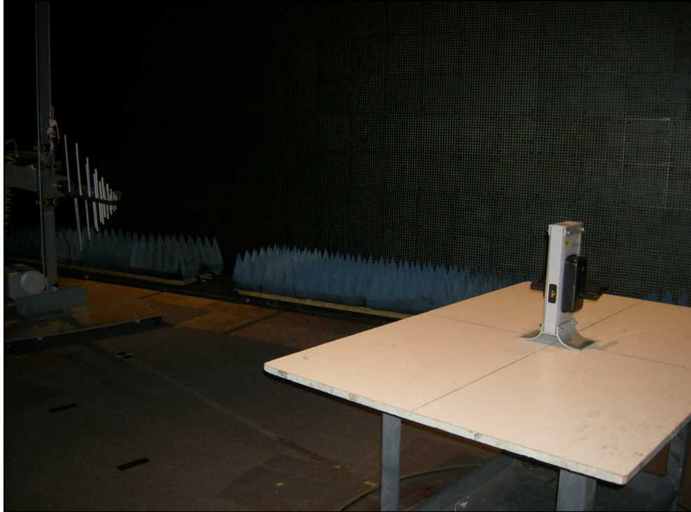
Figure 8: Radiated Emissions – Push Button Lever Lock
