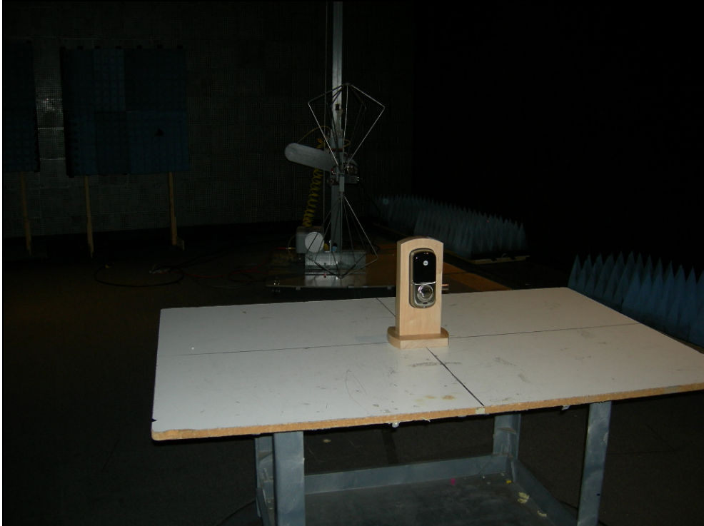
Figure 6: Radiated Emissions – Push Button Deadbolt – YRD210-ZW
