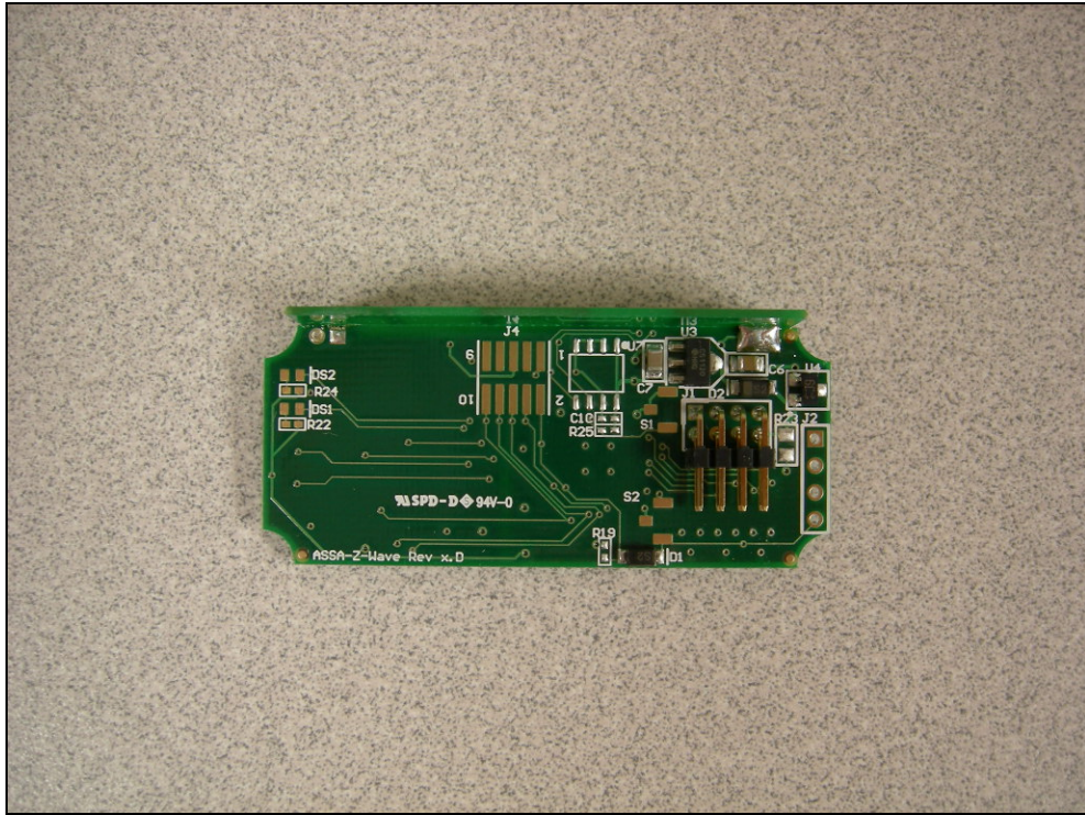
Figure 4: Internal Photo – RF PCB
