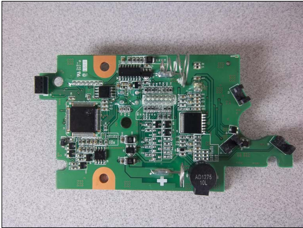
Figure 2: Internal Photo – Main Control PCB
