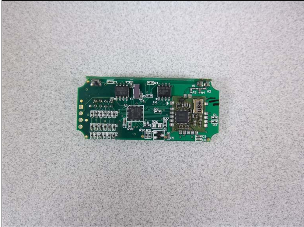
Figure 3: Internal Photo – RF PCB
