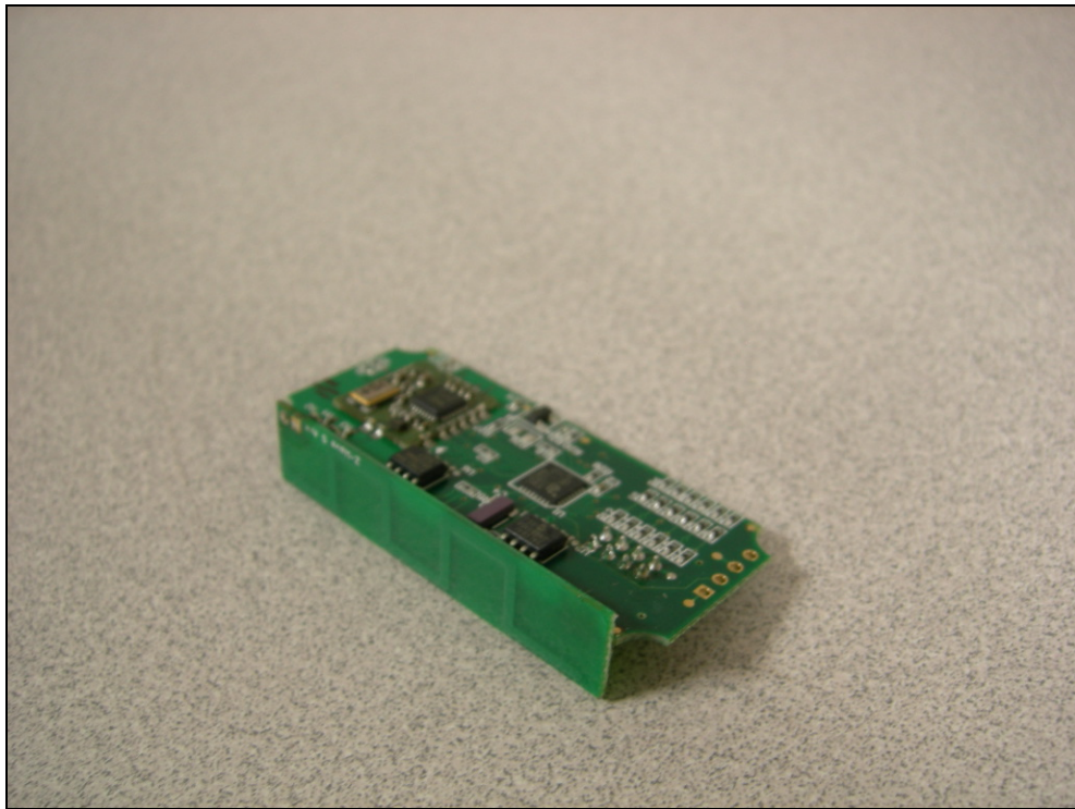
Figure 5: Internal Photo – RF PCB
