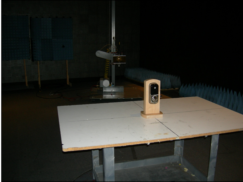
Figure 9: Radiated Emissions – Push Button Deadbolt – YRD210-ZB
