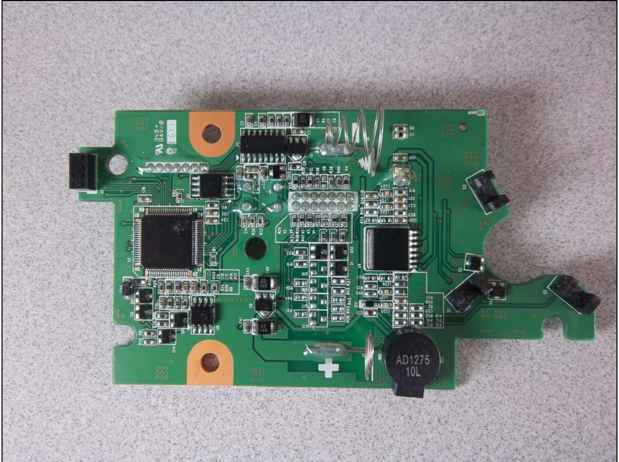
Figure 2: Internal Photo –Main Control PCB
