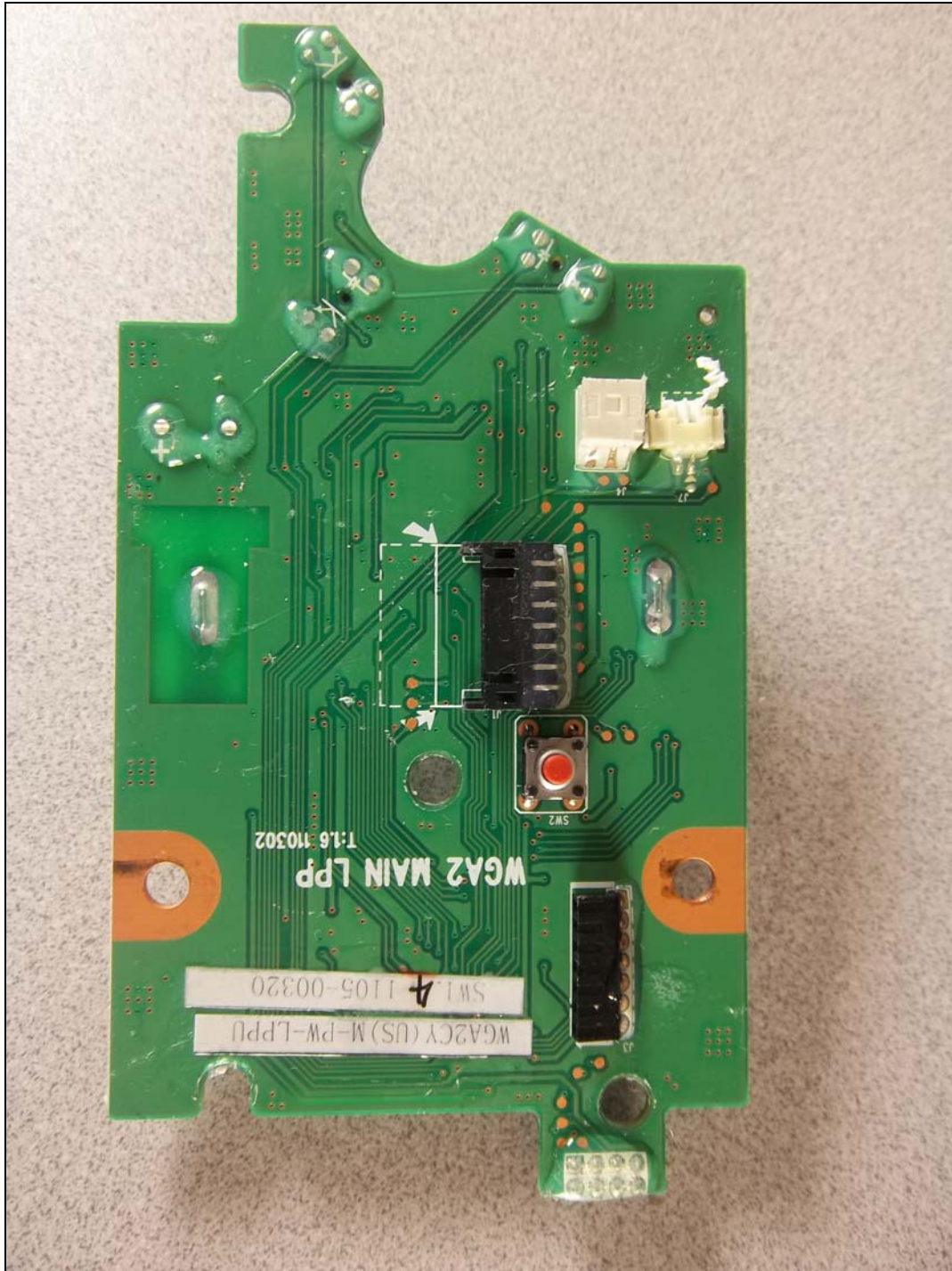
Figure 1: Internal Photo –Main Control PCB
