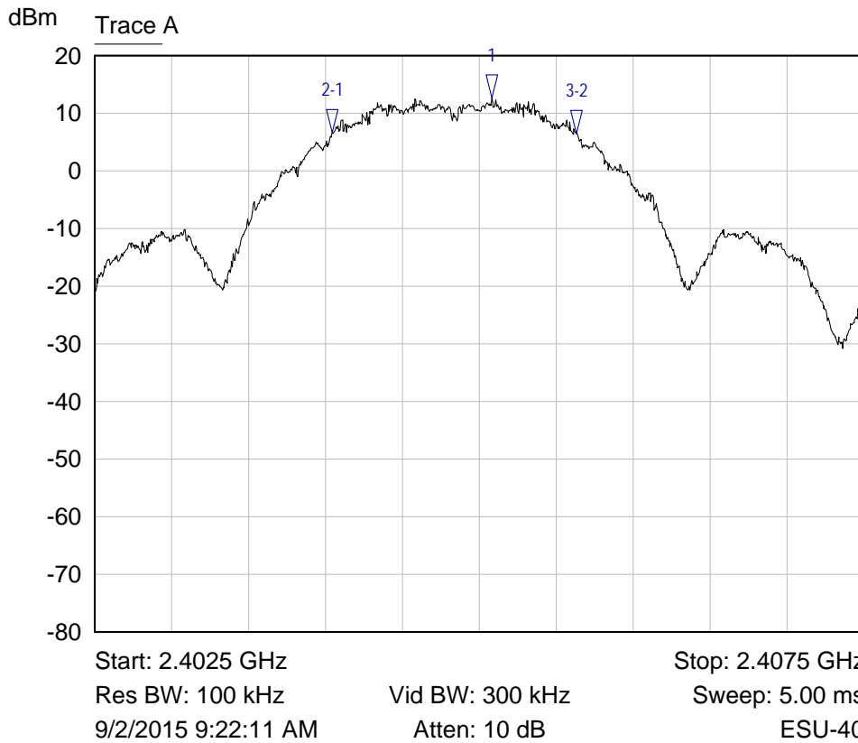
Channel 11 Bandwidth
