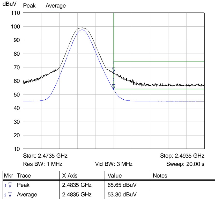
Graph 10: Radiated Upper Band Edge Plot
