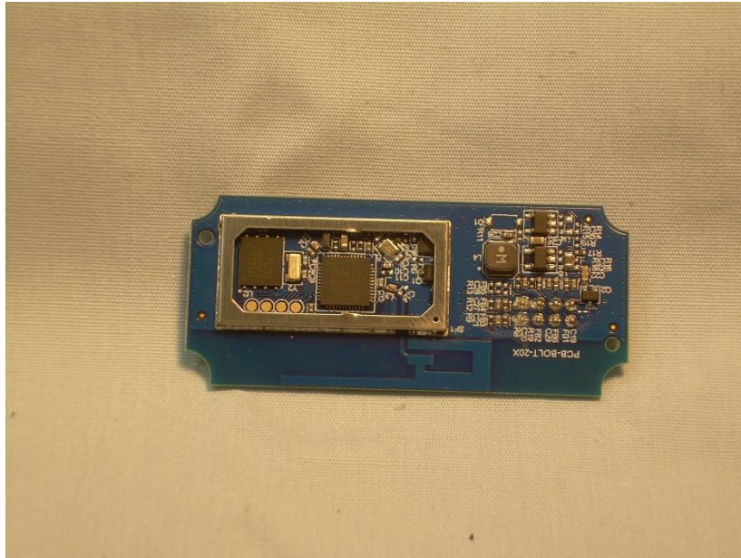
Photograph 15 – Top View of the PCB with RF Cover Removed
