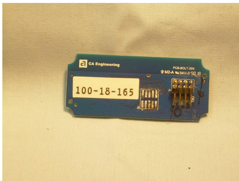
Photograph 17 – Bottom Side of the PCB
