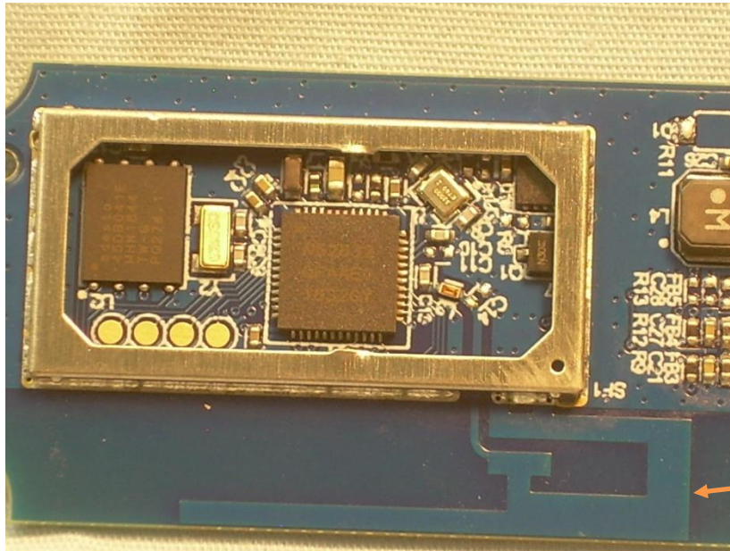
Photograph 16 – View of the Circuitry Under the RF Shield and Antenna
