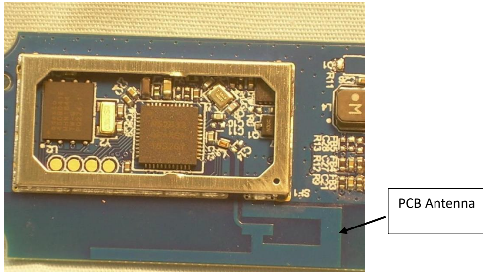
Photograph 3 – View of the Circuitry under the RF Shield
