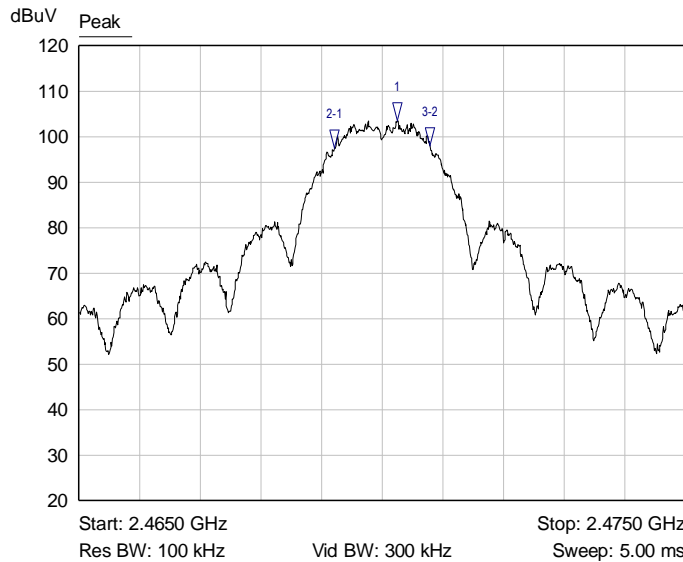
Graph 3: Channel 23 Bandwidth
