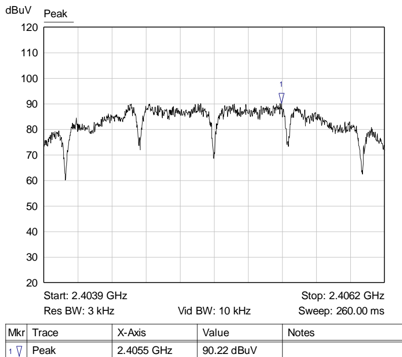
Graph 15: Channel 11 – 3 kHz PSD Plot
