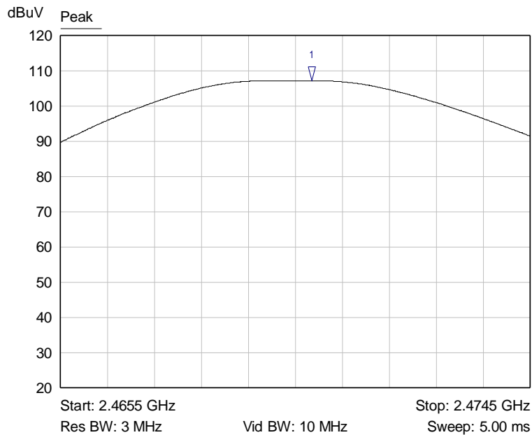
Graph 8: Channel 23 Peak Power Plot
