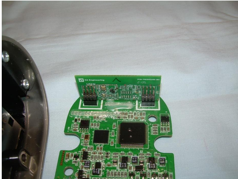
Photograph 11: Transceiver PCB Connected to Main PCB
