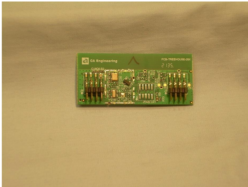
Photograph 12: Connector Side of the Transceiver PCB
