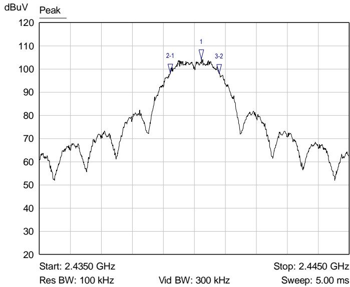
Graph 1: Channel 11 Bandwidth
