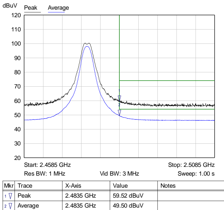
Graph 14: Radiated Upper Band Edge Plot – Channel 25 at Power Setting -f
