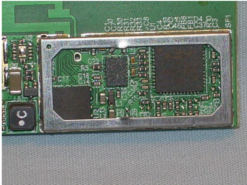
Photograph 14: View of the Circuitry of the Transceiver Under the RF Shield
