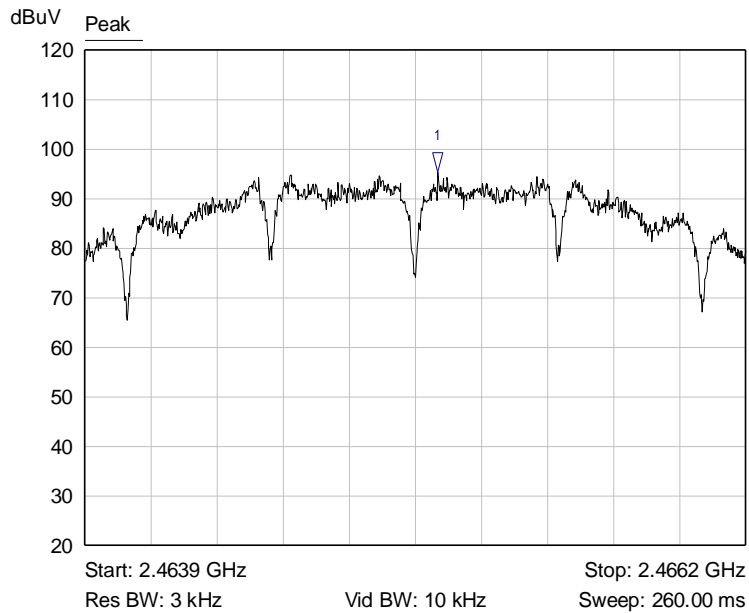
Graph 16: Channel 18 – 3 kHz PSD Plot
