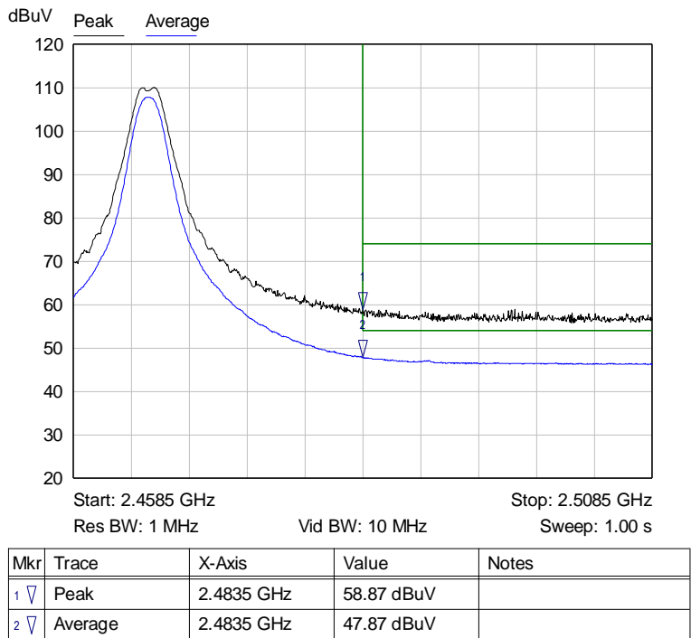
Graph 12: Radiated Upper Band Edge Plot – Channel 23 at Power Setting -5
