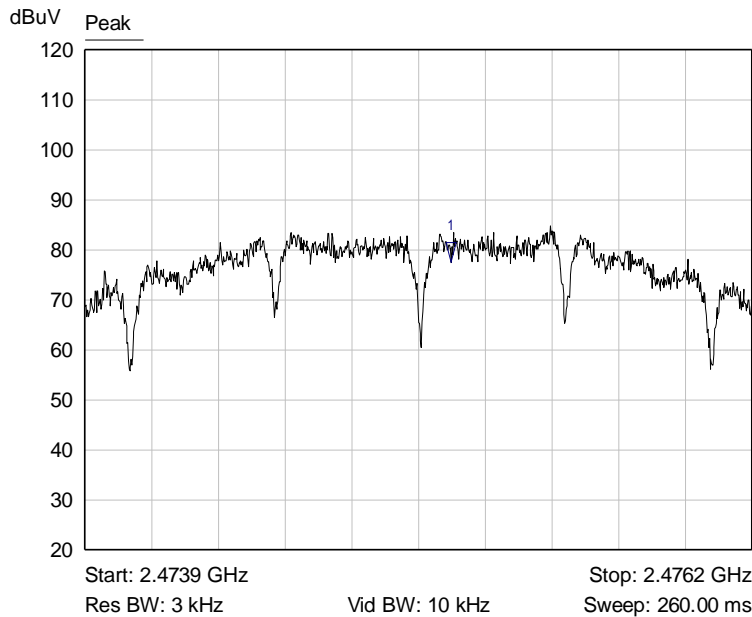
Graph 18: Channel 24 – 3 kHz PSD Plot
