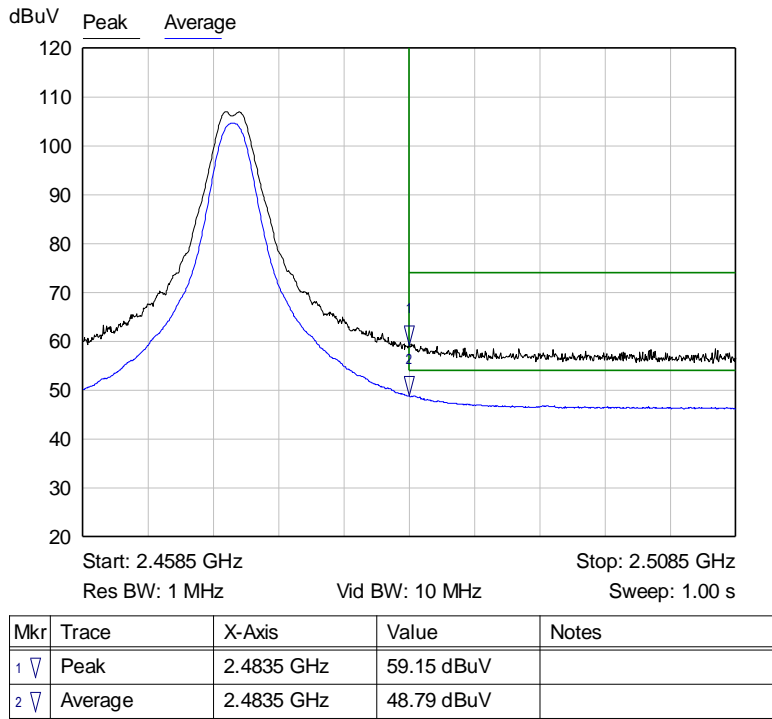
Graph 13: Radiated Upper Band Edge Plot – Channel 24 at Power Setting -9
