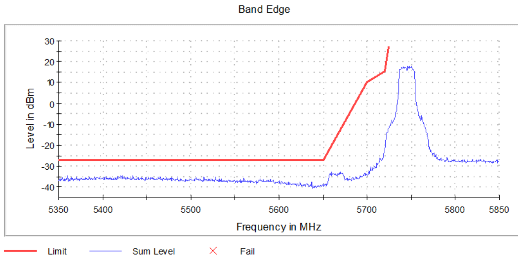
Graph 7: Lower Band Edge Channel 149 Transmitting (5745 MHz)
