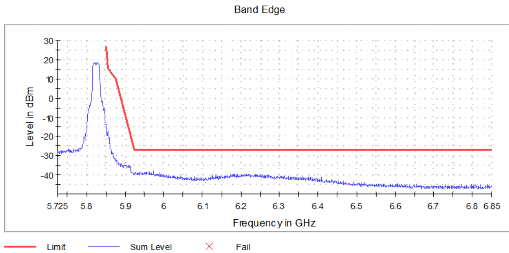
Graph 8: Upper Band Edge Channel 165 Transmitting (5825 MHz)
