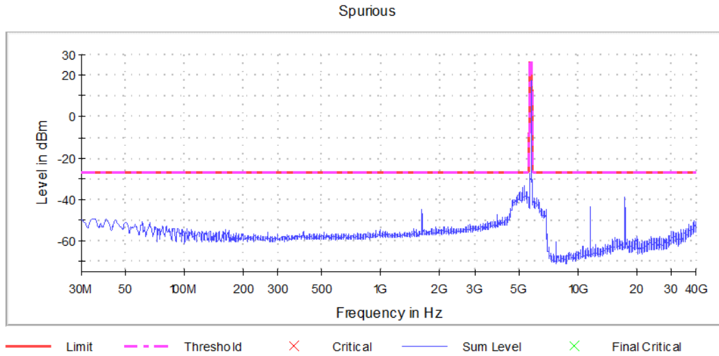
Graph 11: Spurious Emissions Channel 165 Transmitting (5825 MHz)
