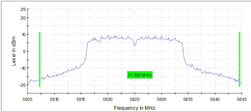
Graph 3: 26 dB Emissions Bandwidth Transmitting at 5825 MHz
