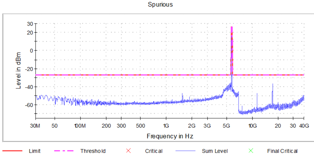
Graph 9: Spurious Emissions Channel 149 Transmitting (5745 MHz)
