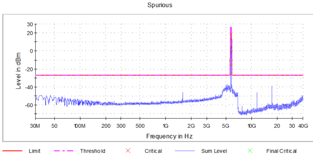
Graph 10: Spurious Emissions Channel 157 Transmitting (5785 MHz)
