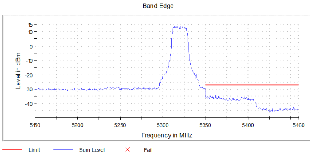
Graph 10: High Band Edge Channel 64 Transmitting (5320 MHz)
