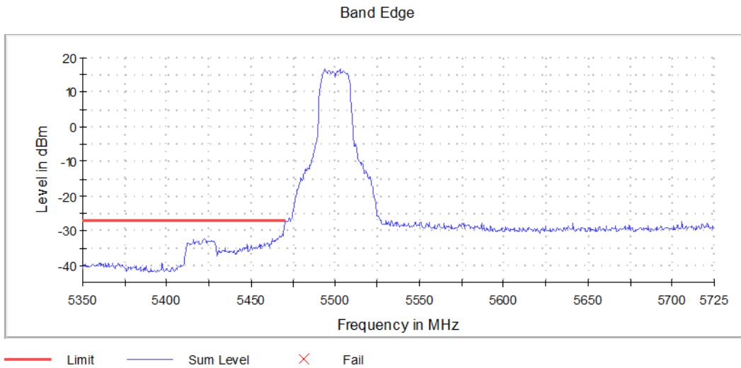
Graph 11: Low Band Edge Channel 100 Transmitting (5500 MHz)
