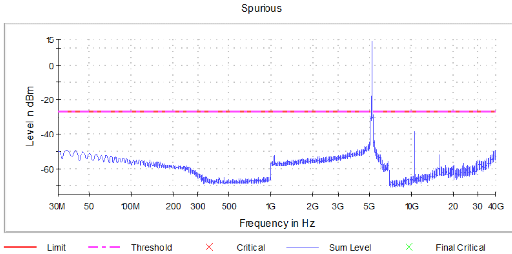
Graph 13: Spurious Emissions Channel 52 Transmitting (5260 MHz)
