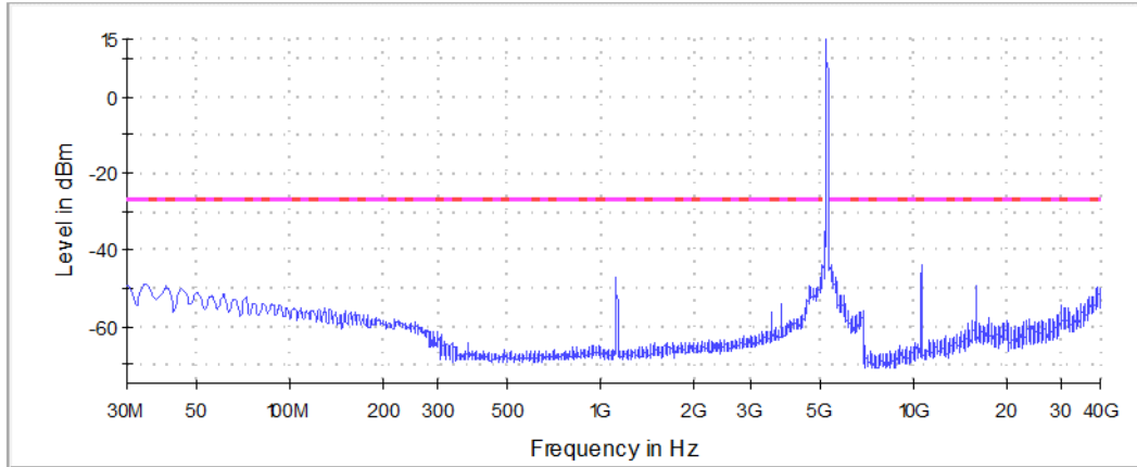
Graph 15: Spurious Emissions Channel 64 Transmitting (5320 MHz)
