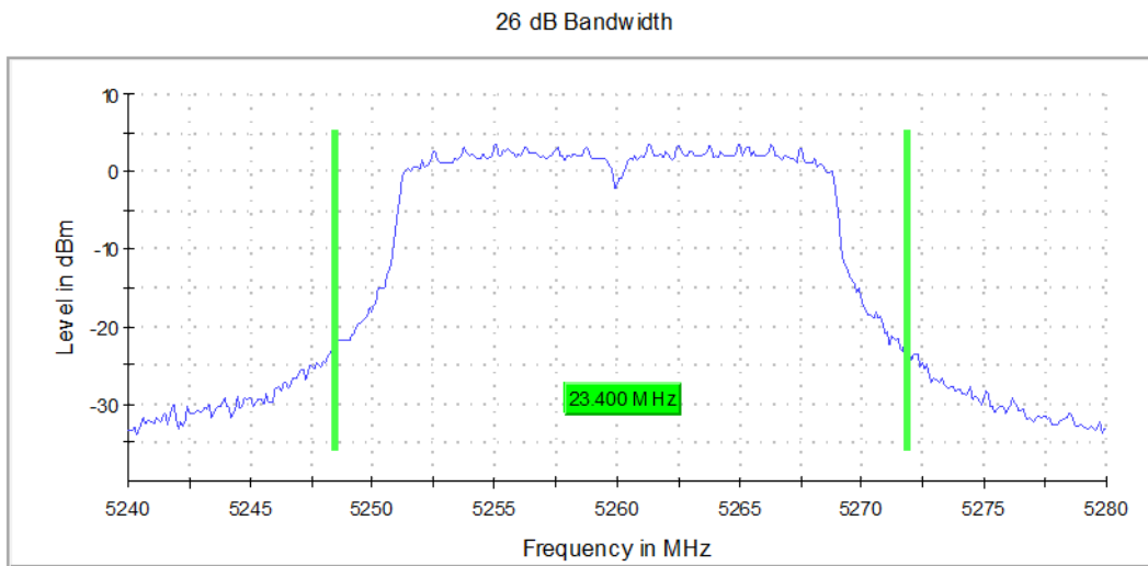
Graph 1: 26 dB Emissions Bandwidth Transmitting at 5260 MHz
