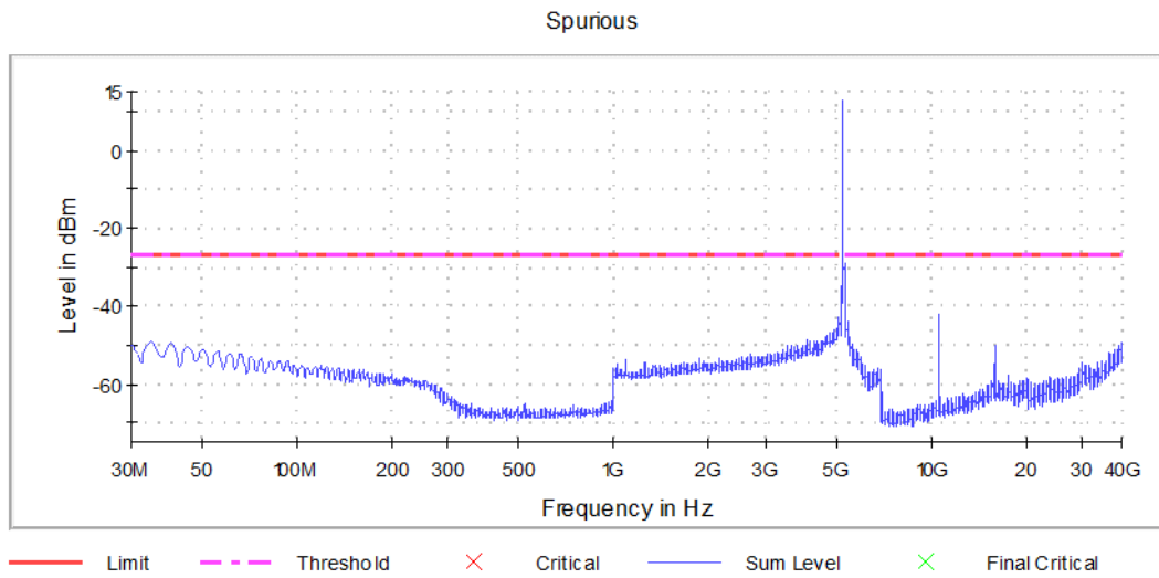
Graph 14: Spurious Emissions Channel 60 Transmitting (5300 MHz)
