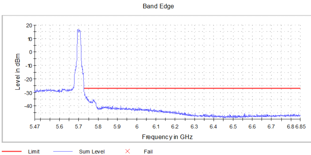
Graph 12: High Band Edge Channel 140 Transmitting (5700 MHz)
