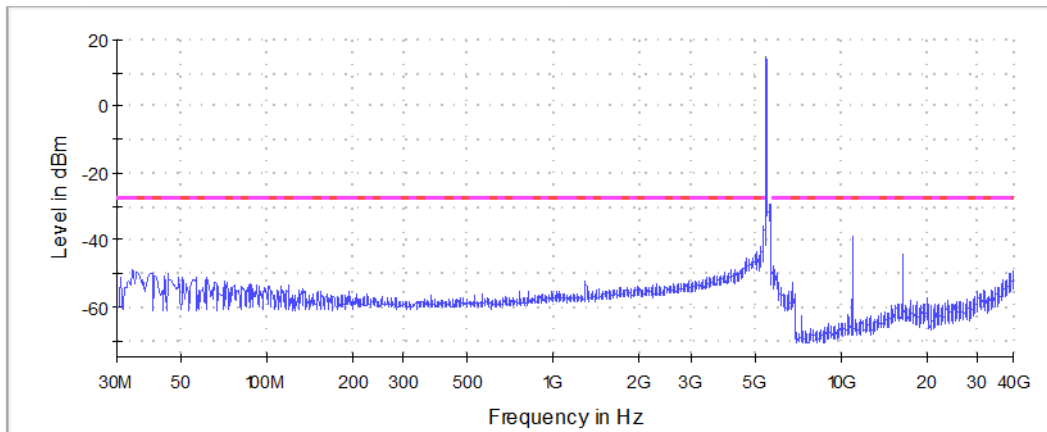
Graph 16: Spurious Emissions Channel 100 Transmitting (5500 MHz)
