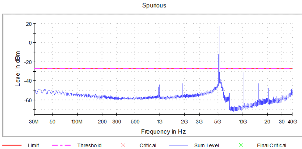
Graph 6: Spurious Emissions Channel 36 Transmitting
