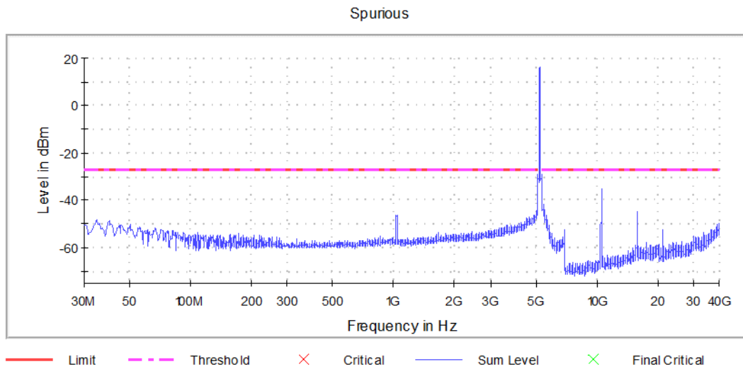
Graph 8: Spurious Emissions Channel 48 Transmitting
