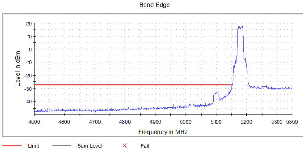
Graph 5: Lower Band Edge Channel 36 Transmitting
