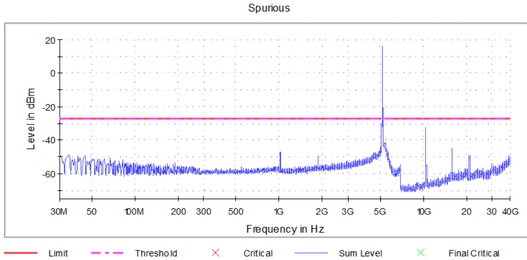
Graph 7: Spurious Emissions Channel 40 Transmitting
