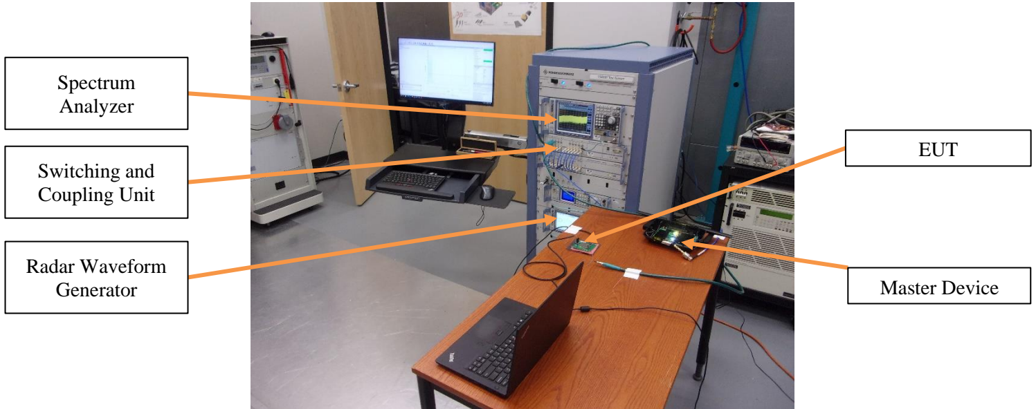
Photograph 1: DFS Test Setup
