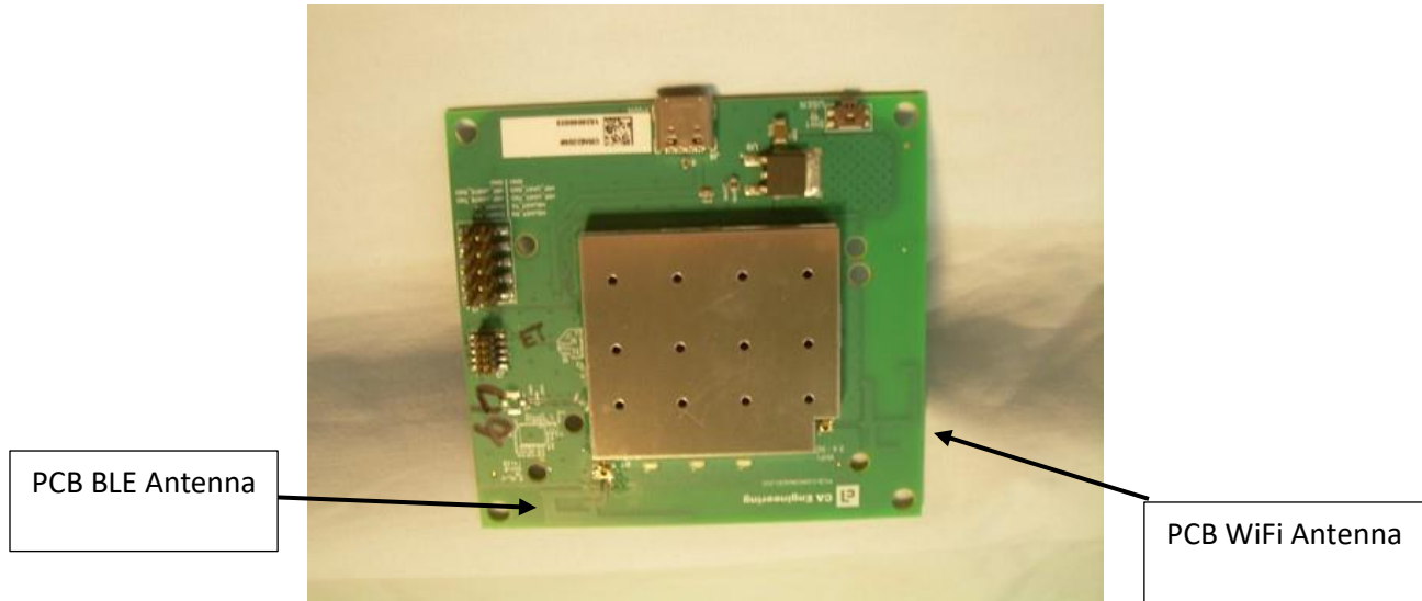
Photograph 1 – Top View of the PCB with Shield
