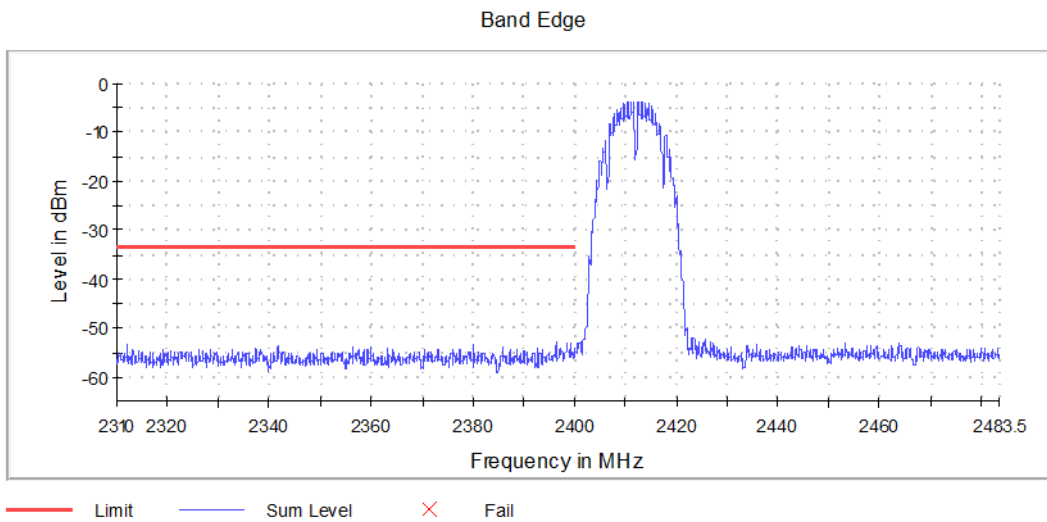
Graph 7: Lower Band Edge Plot
