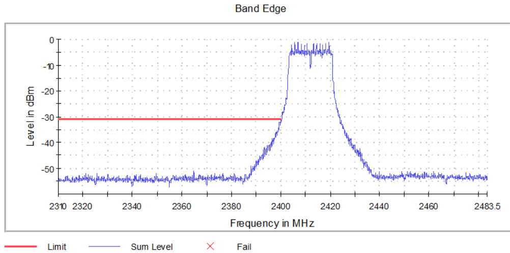
Graph 39: Lower Band Edge Plot
