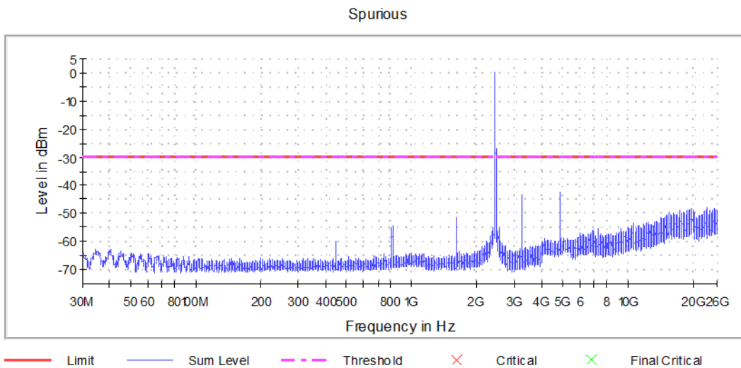
Graph 21: Transmitting on the Middle Channel
