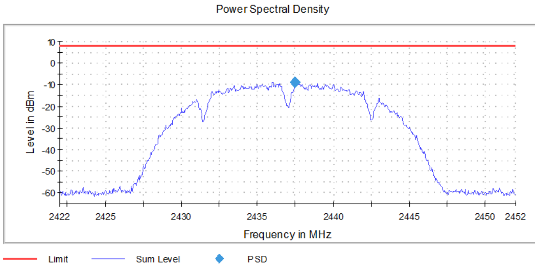
Graph 12: Middle Channel PSD Plot
