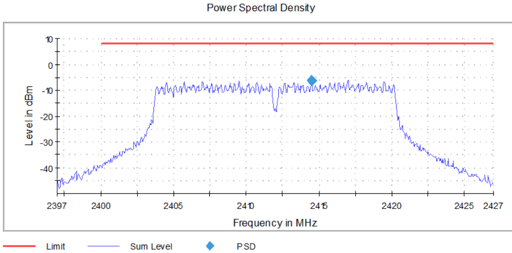
Graph 27: Lowest Channel PSD Plot
