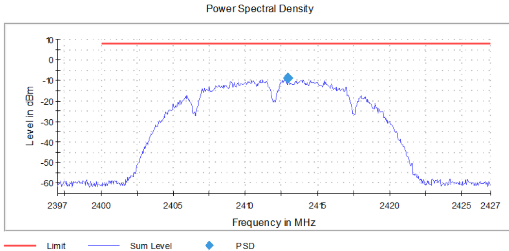
Graph 11: Lowest Channel PSD Plot
