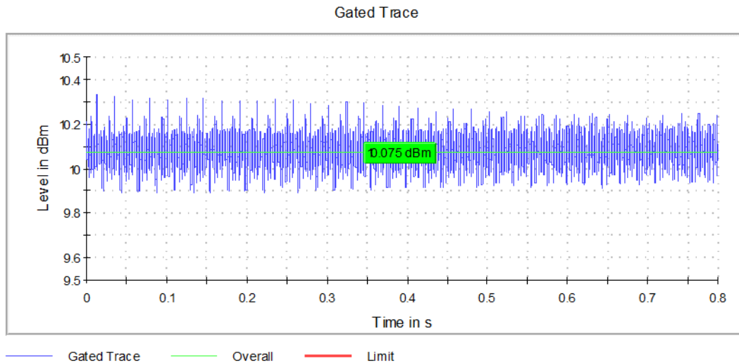
Graph 19: Highest Channel Output Power Plot
