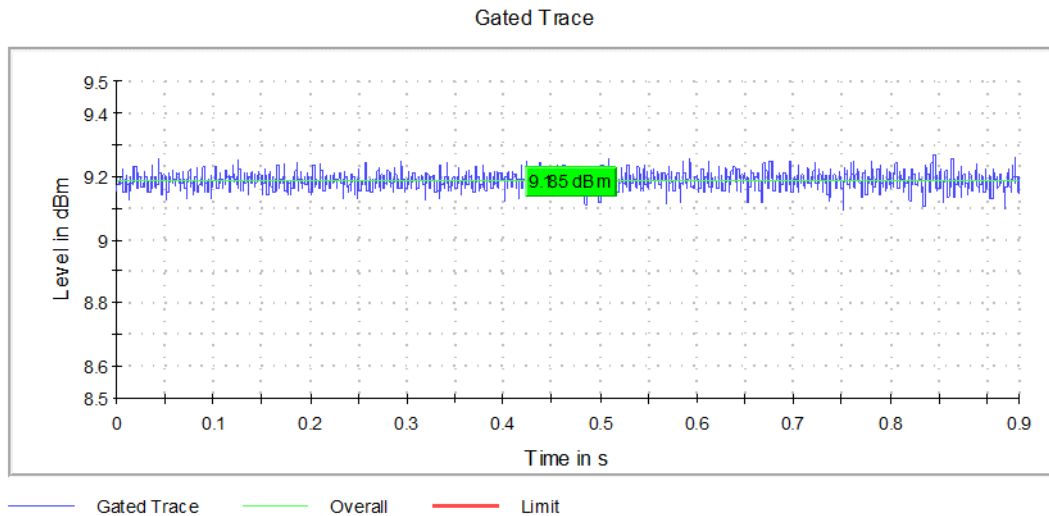
Graph 35: Highest Channel Output Power Plot
