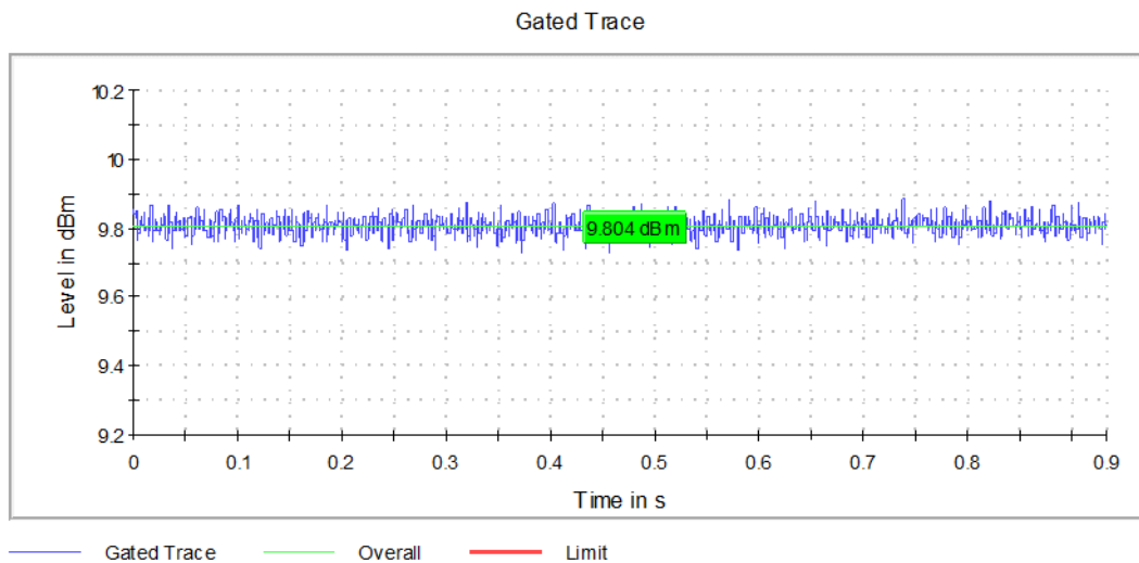
Graph 34: Middle Channel Output Power
