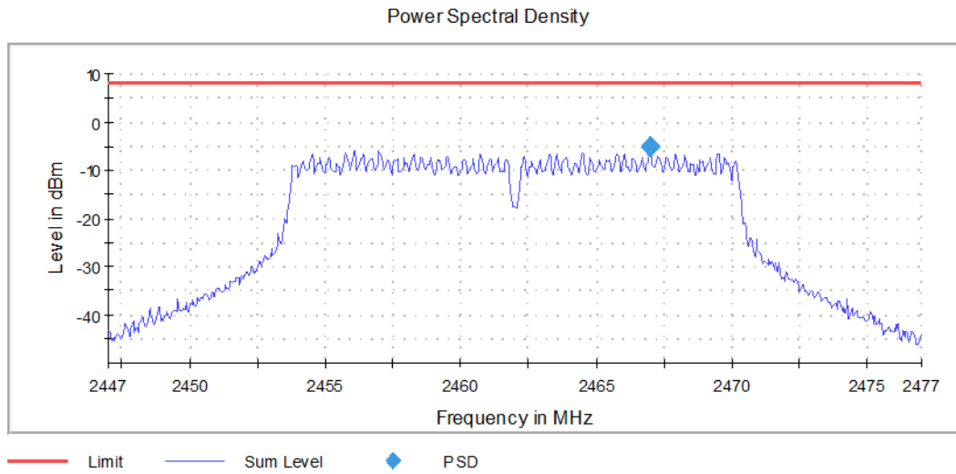
Graph 29: Highest Channel Output PSD Plot
