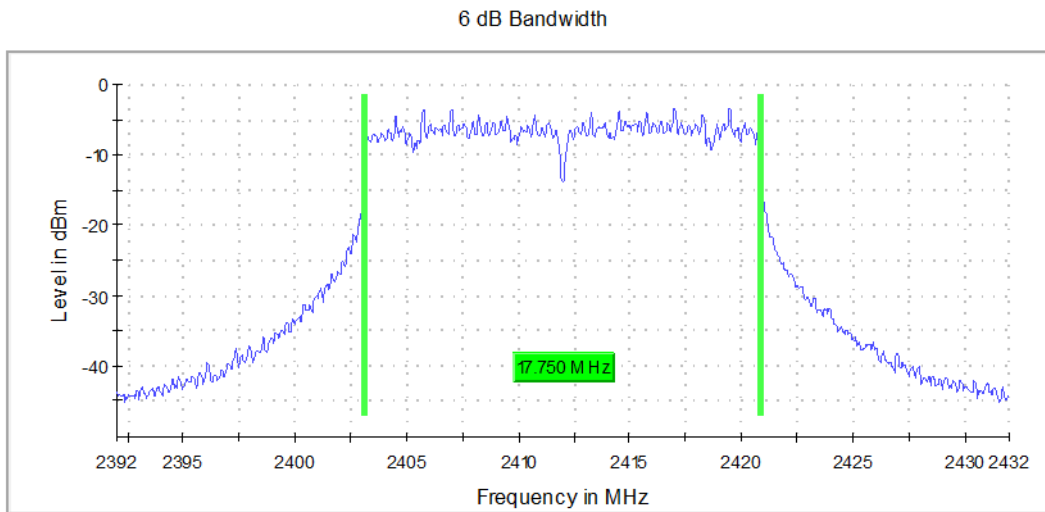
Graph 30: Lowest Channel Bandwidth
