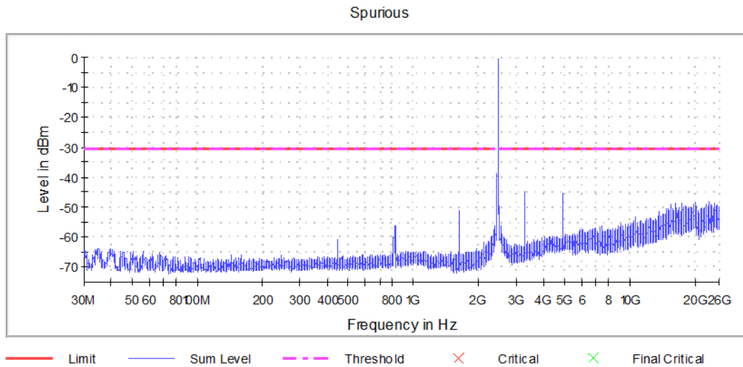
Graph 38: Transmitting on the Highest Channel
