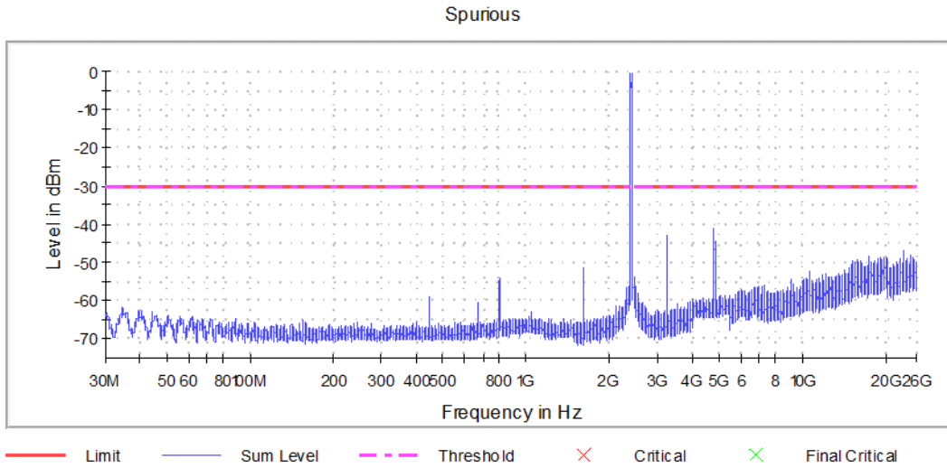
Graph 20: Transmitting on the Lowest Channel
