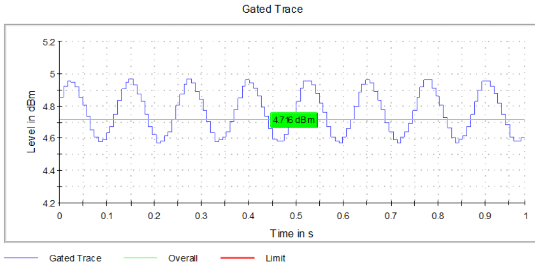
Graph 6: Highest Channel Output Power Plot
