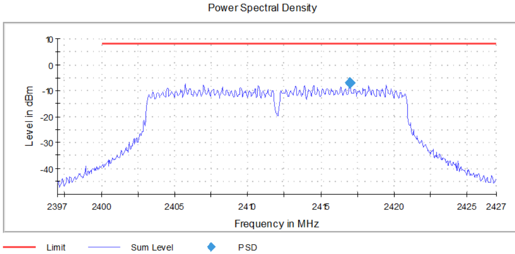
Graph 43: Lowest Channel PSD Plot
