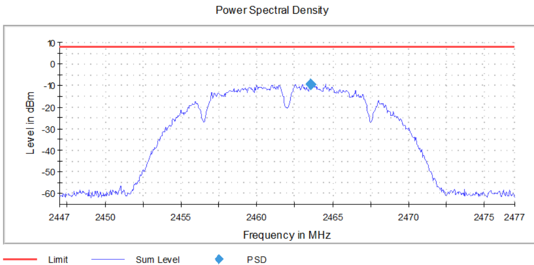
Graph 13: Highest Channel Output 3 PSD Plot
