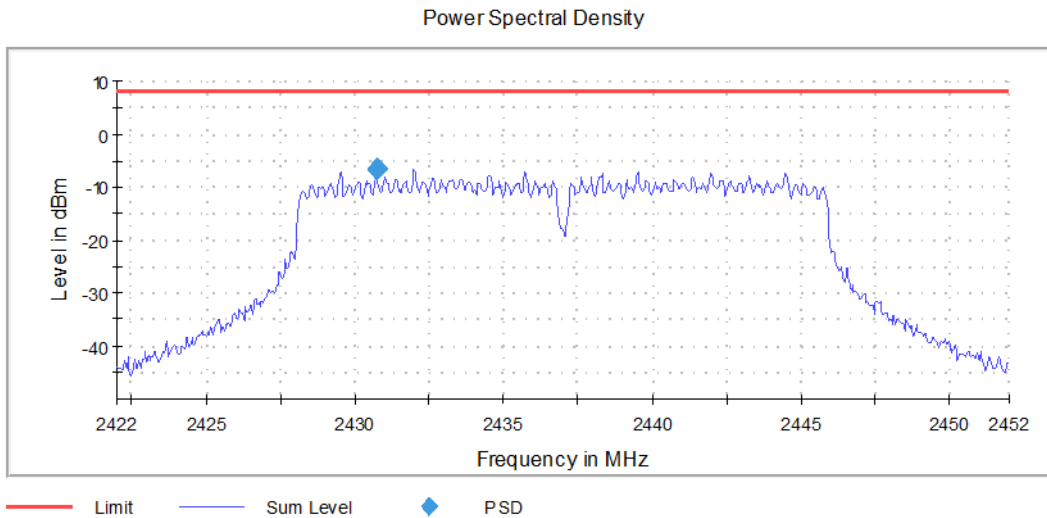
Graph 44: Middle Channel PSD Plot
