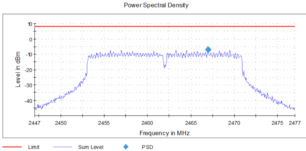
Graph 45: Highest Channel Output PSD Plot
