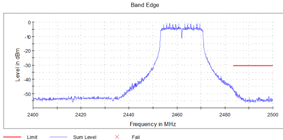
Graph 40: Upper Band Edge Plot
