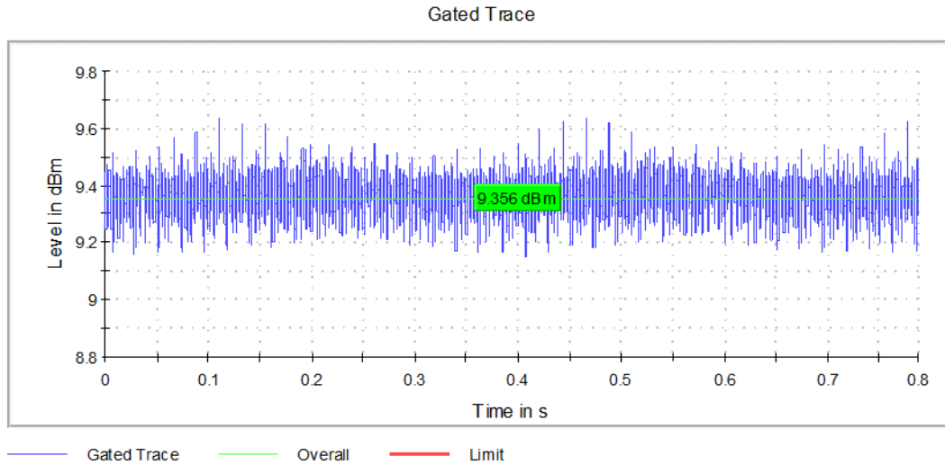
Graph 17: Lowest Channel Output Power Plot
