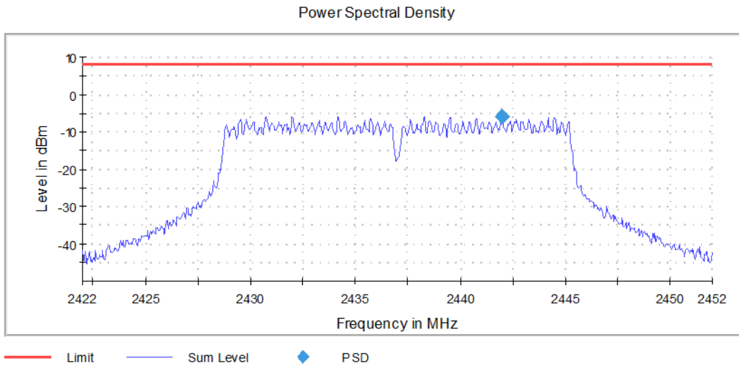
Graph 28: Middle Channel PSD Plot
