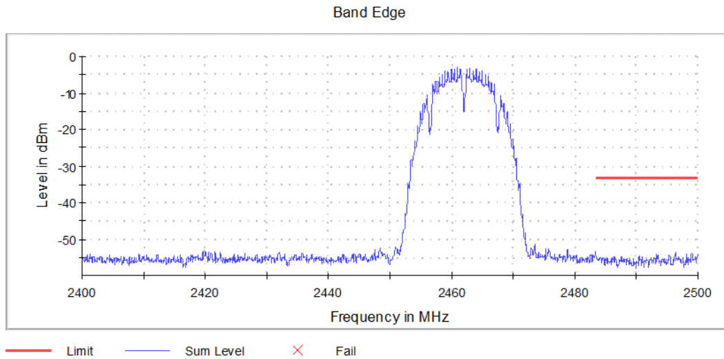
Graph 8: Upper Band Edge Plot
