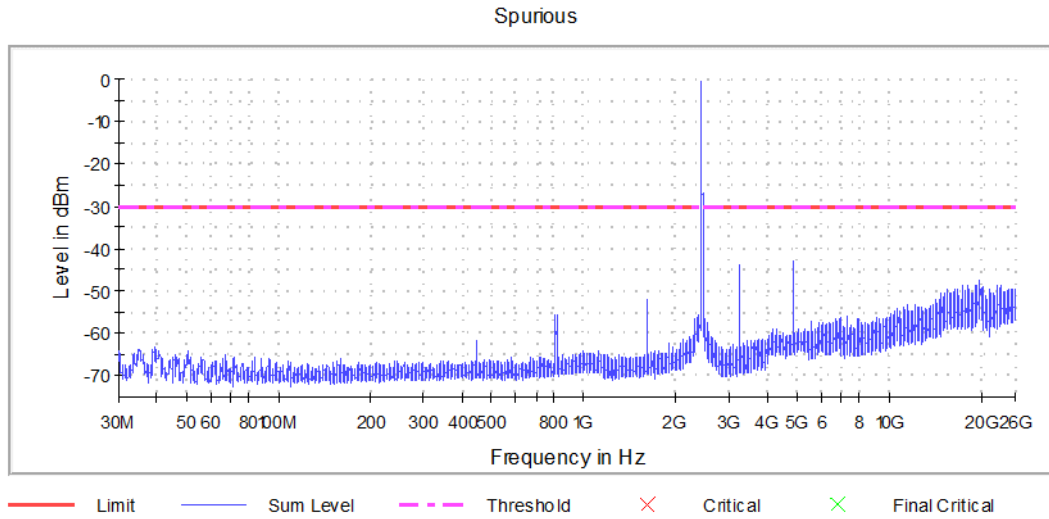
Graph 37: Transmitting on the Middle Channel
