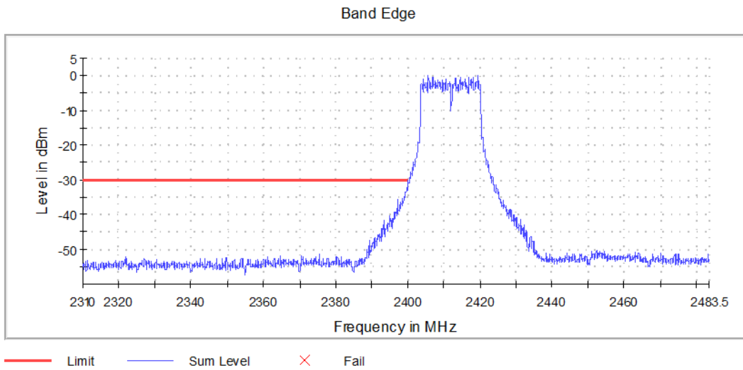
Graph 23: Lower Band Edge Plot
