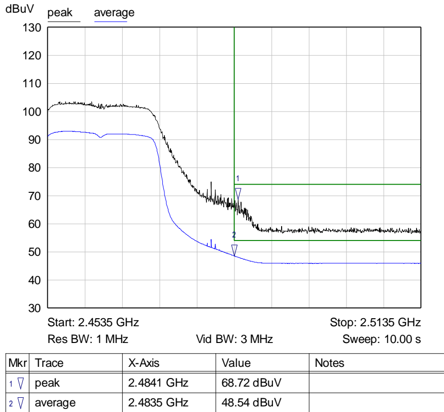
Graph 42: Radiated Upper Band Edge Plot
