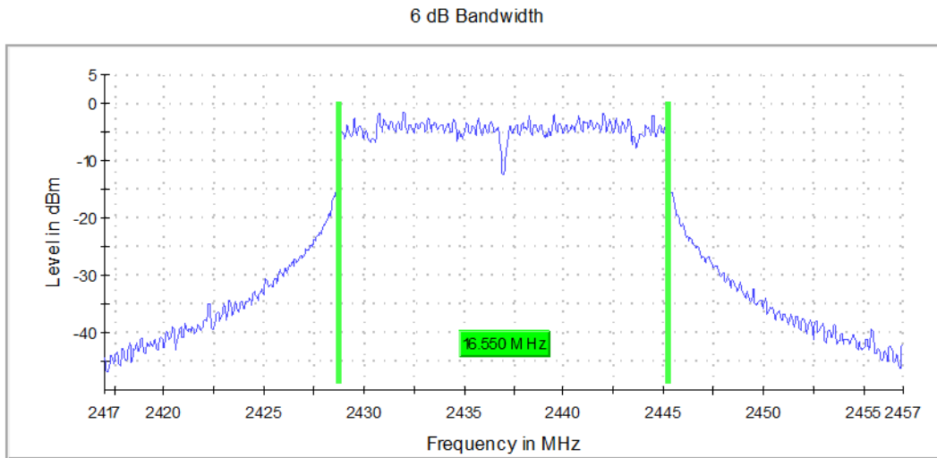
Graph 15: Middle Channel Bandwidth
