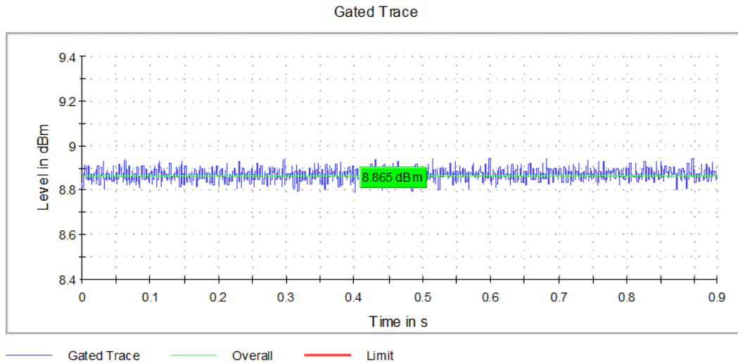
Graph 33: Lowest Channel Output Power Plot
