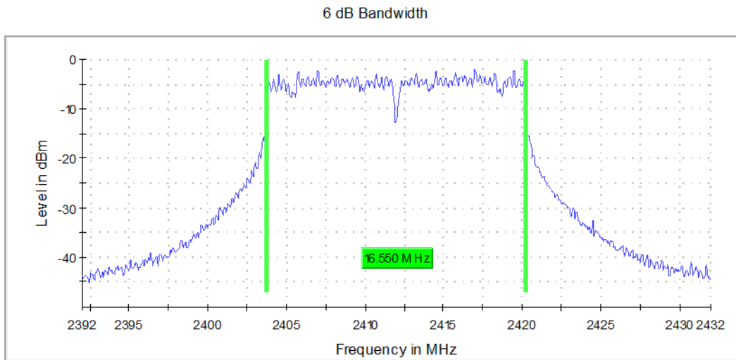
Graph 14: Lowest Channel Bandwidth
