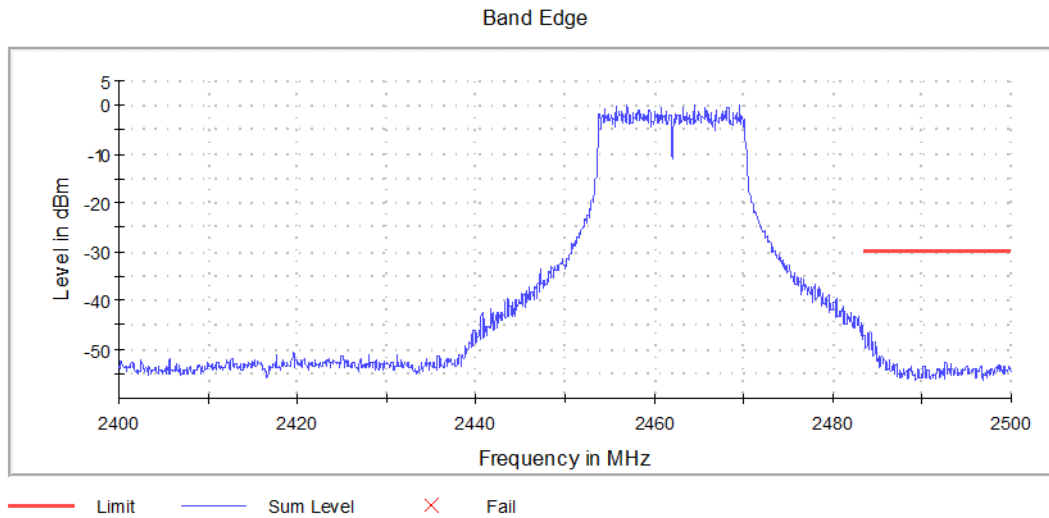
Graph 24: Upper Band Edge Plot
