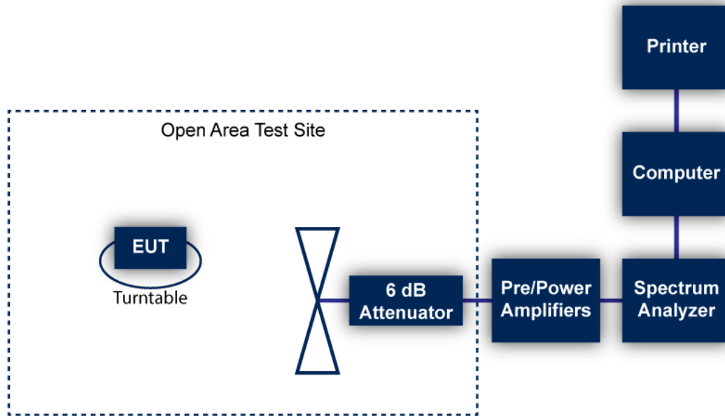
Figure 3: Radiated Emissions Test
