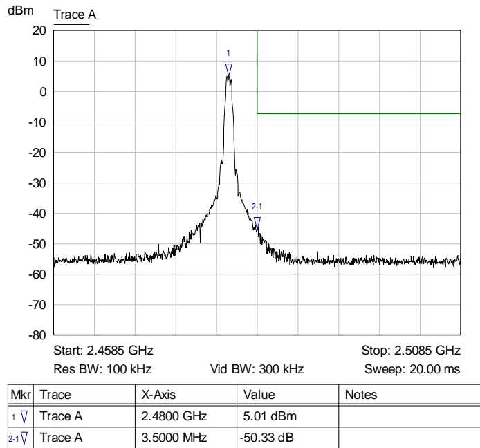
Graph 8: Upper Band Edge Plot
