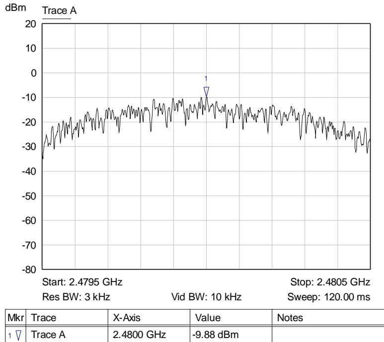
Graph 13: Upper Channel 3 kHz PSD Plot
