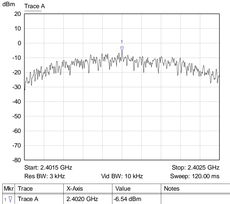
Graph 11: Lowest Channel 3 kHz PSD Plot
