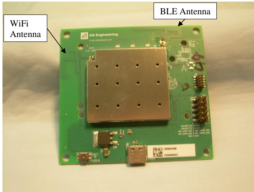
Photograph 12: Top Side of the PCB
