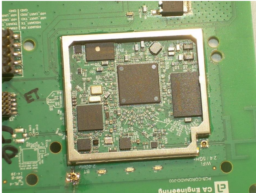
Photograph 14: Circuitry Under the RF Shield
